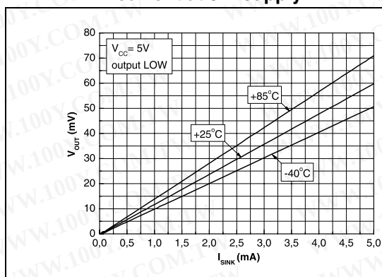
Figure 4. Output voltage versus output current at 5 V supply
