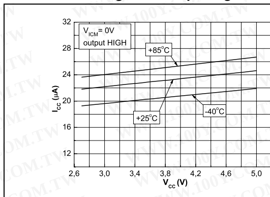
Figure 2. Supply current versus supply voltage with output high
