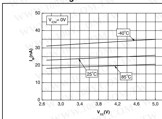
Figure 6. Input bias current versus supply voltage
