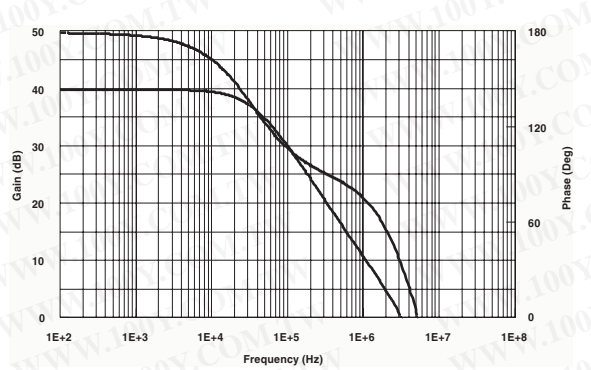
Figure 12. Open loop gain and phase vs. frequency
