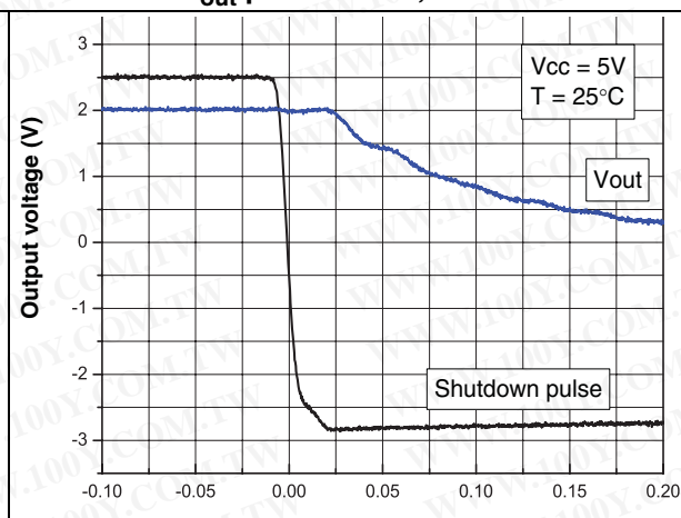
Figure 22. Turn-off time, V_{CC} = 5 V, V_{out} pulled down, T = 25^\circ C
