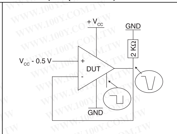
Figure 20. Test configuration for turn-off time (Vout pulled down)
