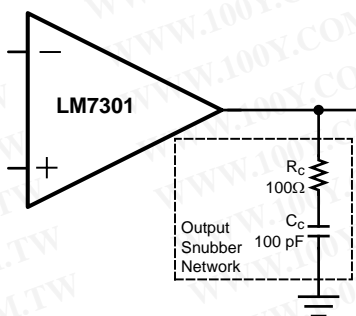
Figure 30. Non-dissipating Snubber Network to Reduce Gain Peaking
