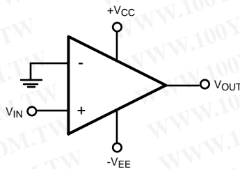
Figure 54. Non-Inverting Comparator
