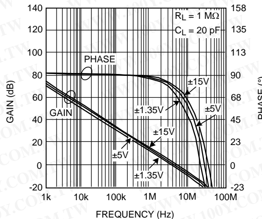
Figure 1. Open Loop Frequency Response
