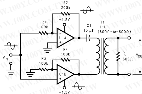
Figure 43. Differential Driver
