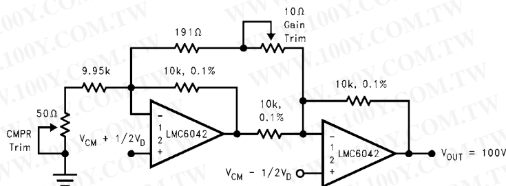
Figure 2. Low-Power Two-Op-Amp Instrumental Amplifier
