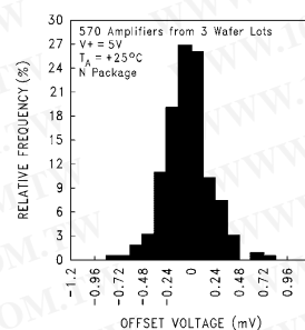
Figure 2. Distribution of LMC6061 Input Offset Voltage ( T_A = +25^\circ\text{C} )
