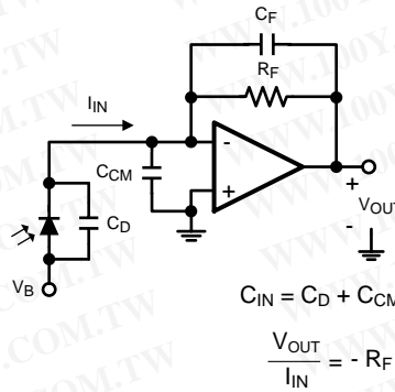
Figure 54. Transimpedance Amplifier
