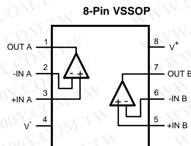
Figure 4. Top View
