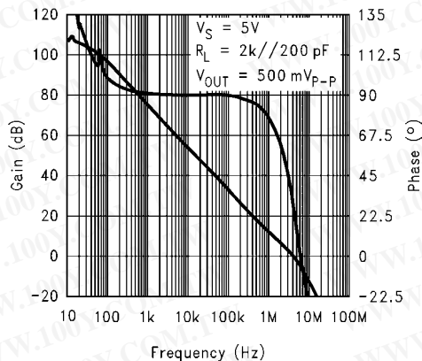
Figure 3. Gain/Phase
