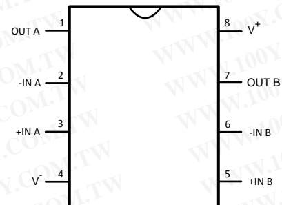
Figure 5. LMV762/LMV762Q (Dual) 8-Pin SOIC and VSSOP Top View
