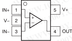
DBV PACKAGE: OPA171 SOT23-5 (TOP VIEW)
