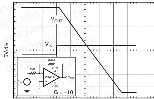
Time (5µs/div)
