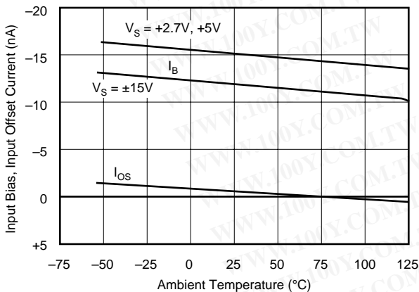
INPUT BIAS AND INPUT OFFSET CURRENT vs TEMPERATURE
