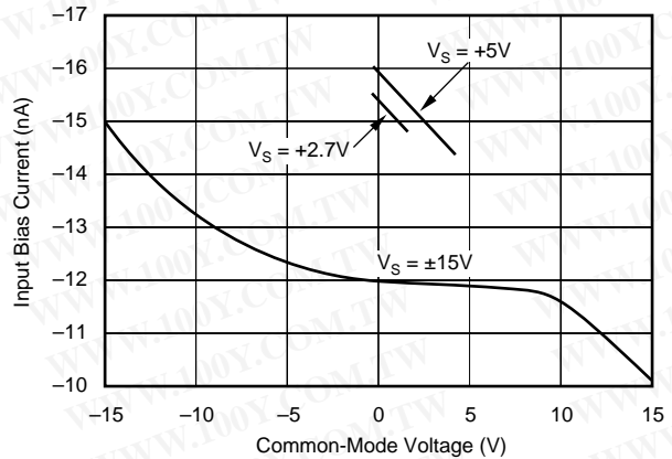
INPUT BIAS CURRENT vs INPUT COMMON-MODE VOLTAGE
