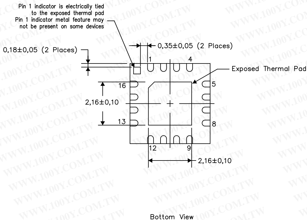
Exposed Thermal Pad Dimensions
