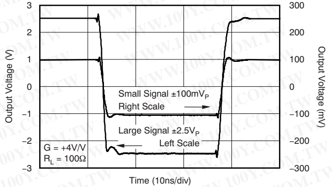
SMALL-SIGNAL AND LARGE-SIGNAL PULSE RESPONSES
