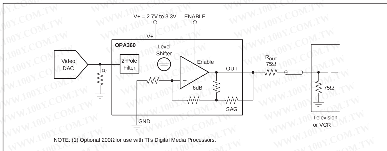
Figure 15. DC-Coupled Input/DC-Coupled Output
