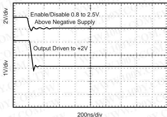
DISABLE (10 \Omega Load)
