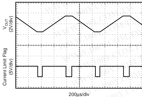
IN AND OUT OF CURRENT LIMIT TRANSIENT ( R_L = 0.75\Omega , Current Limit = 2A)
