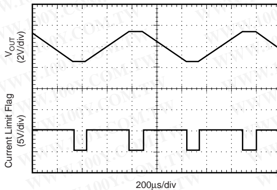
IN AND OUT OF CURRENT LIMIT TRANSIENT ( R_L = 7.5\Omega , Current Limit = 200mA)
