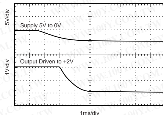
POWER OFF (1 \Omega Load)
