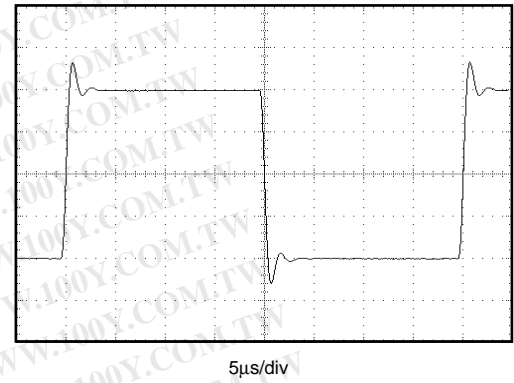
OPA704 SMALL SIGNAL STEP RESPONSE ( G = +5\text{V/V} , C_F = 3\text{pF} , R_F = 100\text{k}\Omega , C_L = 100\text{pF} , R_L = 20\text{k}\Omega )
