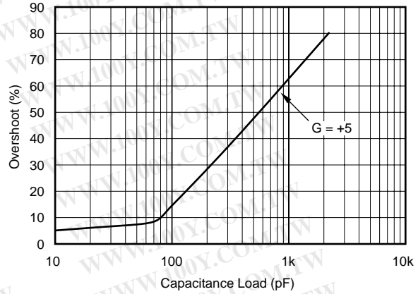
OPA704 SMALL-SIGNAL OVERSHOOT (%) vs CAPACITIVE LOAD
