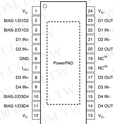
HTSSOP-24 (4) PWP PACKAGE (TOP VIEW)
