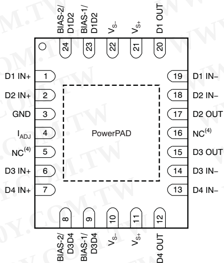
QFN-24 (4) RHF PACKAGE (TOP VIEW)
