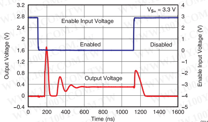
SD ENABLE/DISABLE RESPONSE vs TIME
