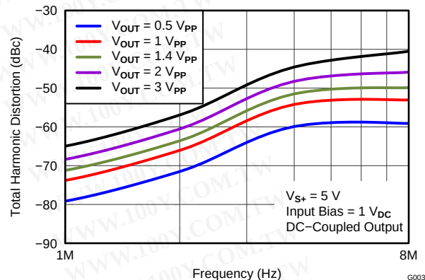
SD THD vs FREQUENCY
