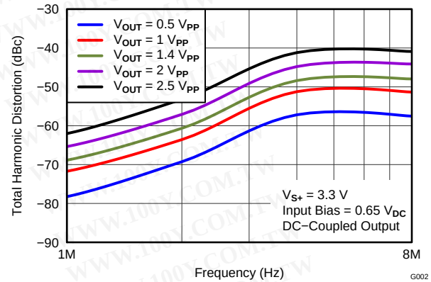
SD THD vs FREQUENCY
