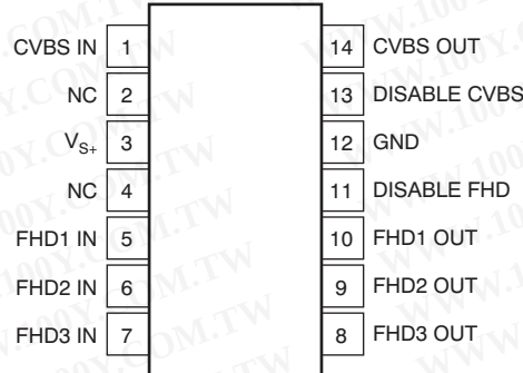
PW PACKAGE TSSOP-14 (TOP VIEW)
