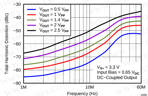
FHD THD vs FREQUENCY
