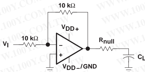
Figure 54. Series-Resistance Circuit
