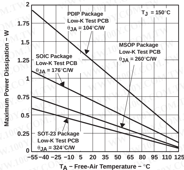
Figure 63. Maximum Power Dissipation vs Free-Air Temperature
