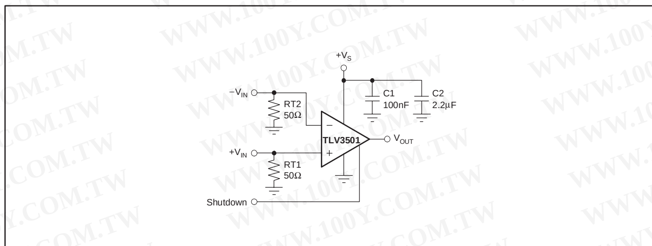
Figure 9. Schematic for Figure 7 and Figure 8
