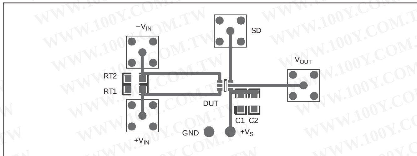
Figure 8. TLV3501DBV (SOT23) Sample Layout
