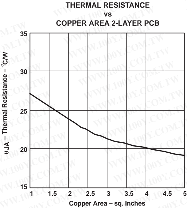
Figure 47. Thermal Resistance
