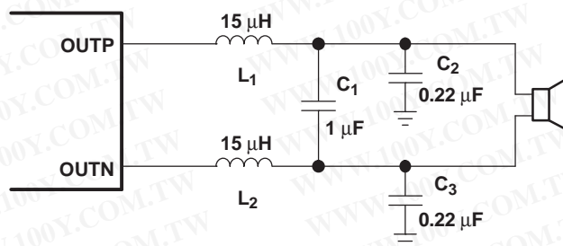
Figure 39. Typical LC Output Filter, Cutoff Frequency of 27 kHz, Speaker Impedance = 4 Ω
