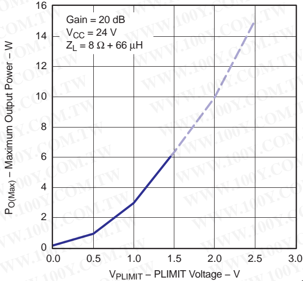
NOTE: Dashed line represents thermally limited region. Figure 14.
