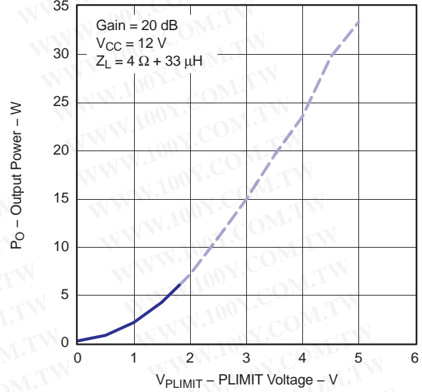
NOTE: Dashed line represents thermally limited region. Figure 15.
