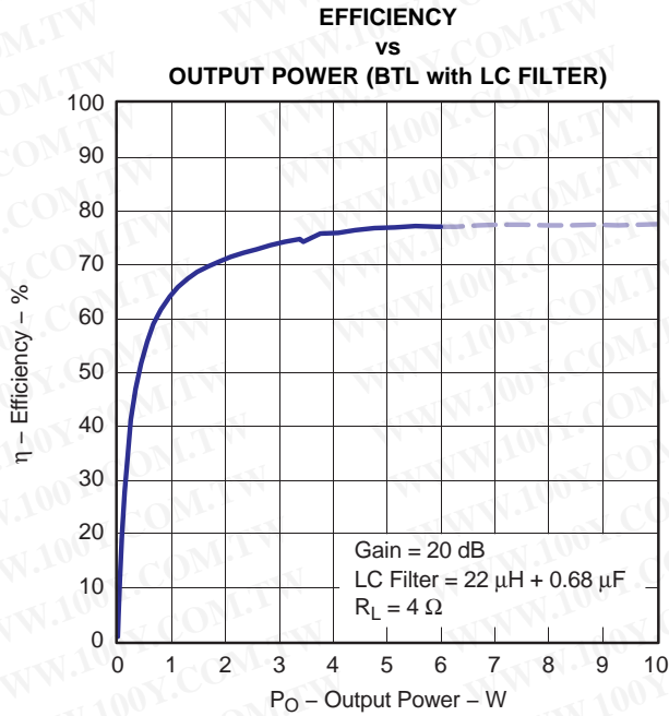
NOTE: Dashed line represents thermally limited region. Figure 22.
