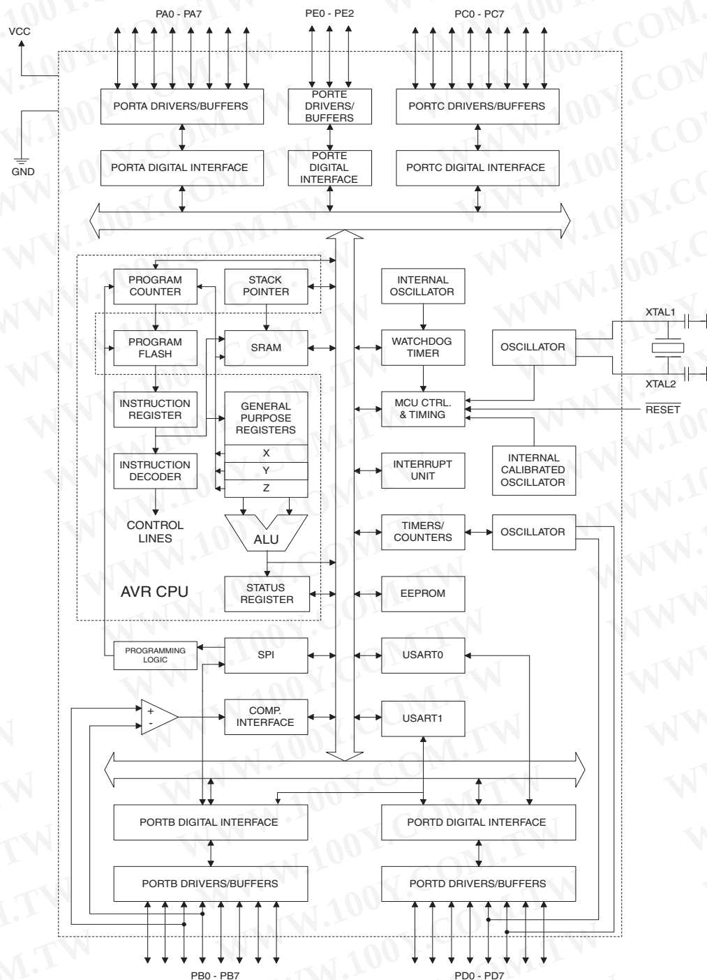
Figure 2. Block Diagram
