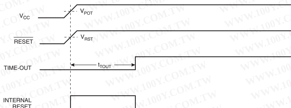
Figure 10-2. MCU Start-up, \overline{RESET} Tied to V_{CC} .
