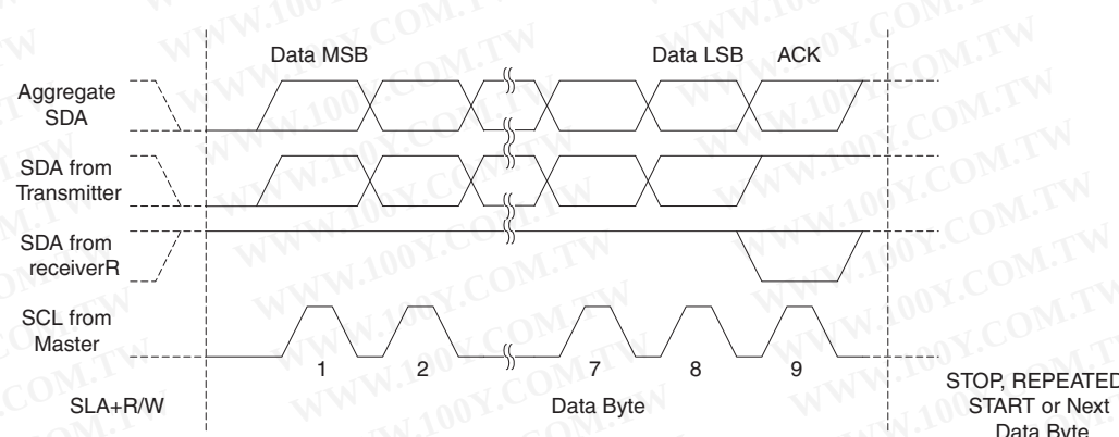
Figure 20-5. Data Packet Format
