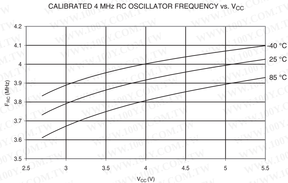
Figure 28-39. Calibrated 4 MHz RC Oscillator Frequency vs. V CC
