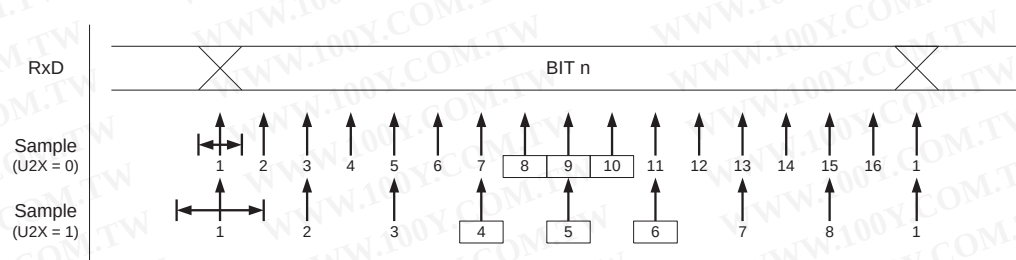
Figure 19-6. Sampling of Data and Parity Bit
