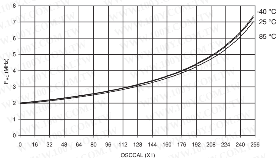
Figure 28-41. Calibrated 2 MHz RC Oscillator Frequency vs. Temperature
