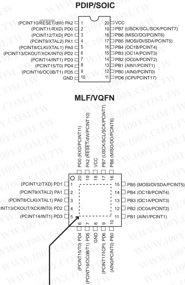
Figure 1-1. Pinout ATtiny2313A/4313
