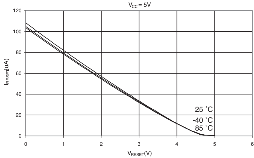
Figure 24-18. Reset Pull-up Resistor Current vs. Reset Pin Voltage ( V_{CC} = 5V )
