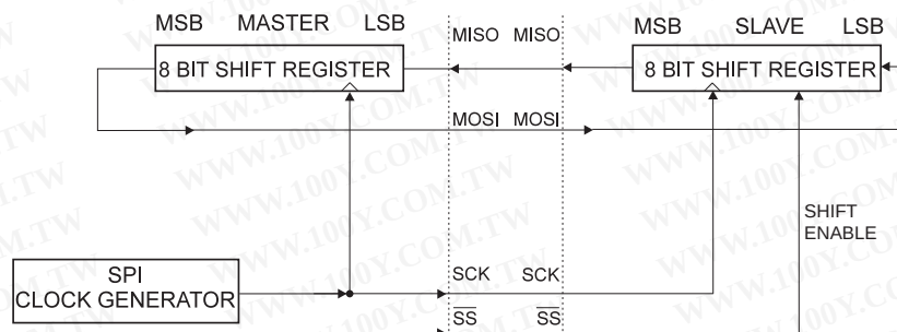
Figure 17-2. SPI Master-slave Interconnection
