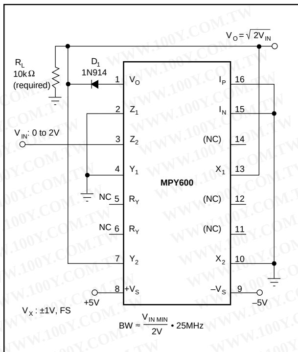
FIGURE 8. Square-Root Circuit.
