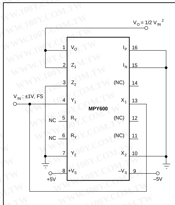
FIGURE 9. Squaring Circuit.
