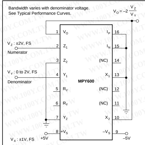
FIGURE 7. Divider Circuit.
