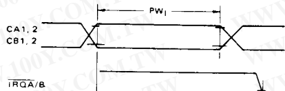
FIGURE 13 — INTERRUPT PULSE WIDTH AND IRQ RESPONSE
