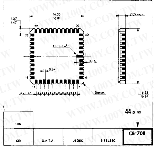
E SUFFIX LCC 44
