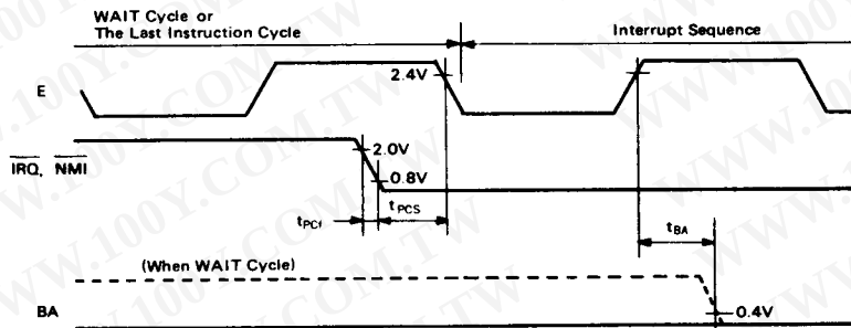
Figure 9 \overline{\text{IRQ}} and \text{NMI} Interrupt Timing
