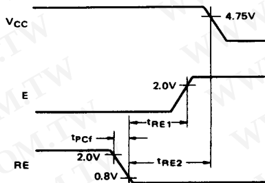
Figure 12 Power-down Sequence
