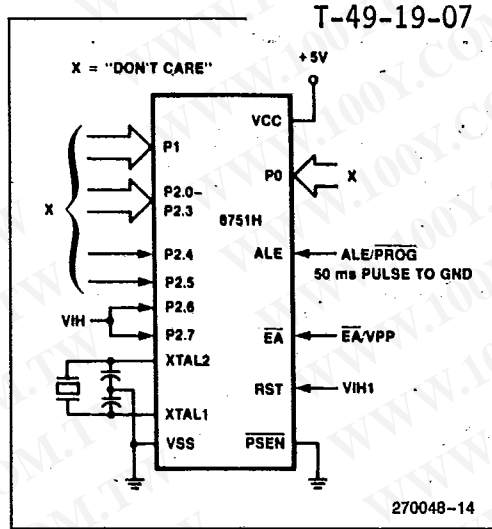
Figure 7. Programming the Security Bit
