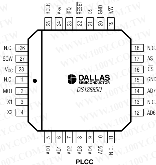
PLCC
