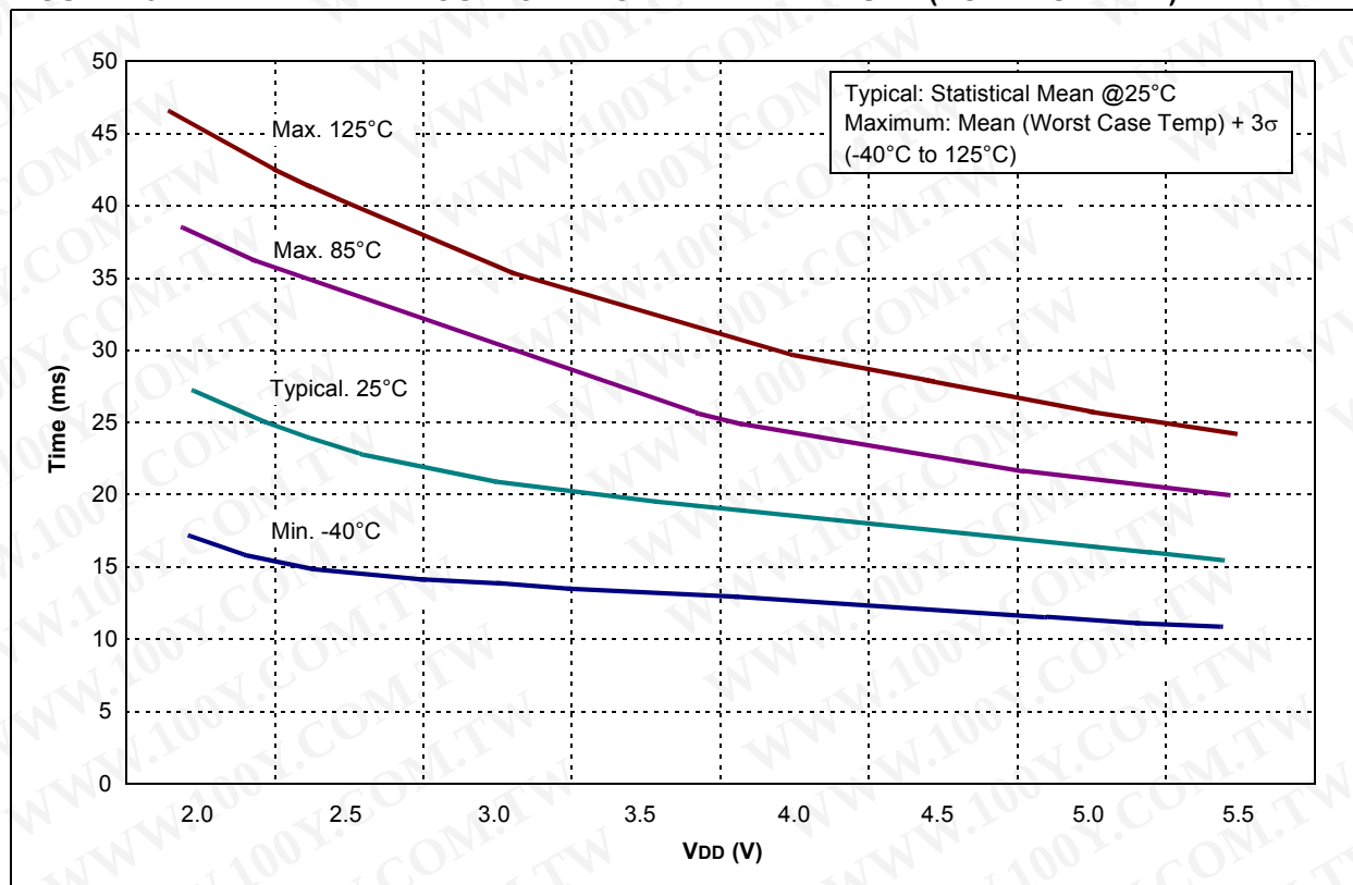
FIGURE 13-7: WDT TIME-OUT vs. V DD OVER TEMPERATURE (NO PRESCALER)
