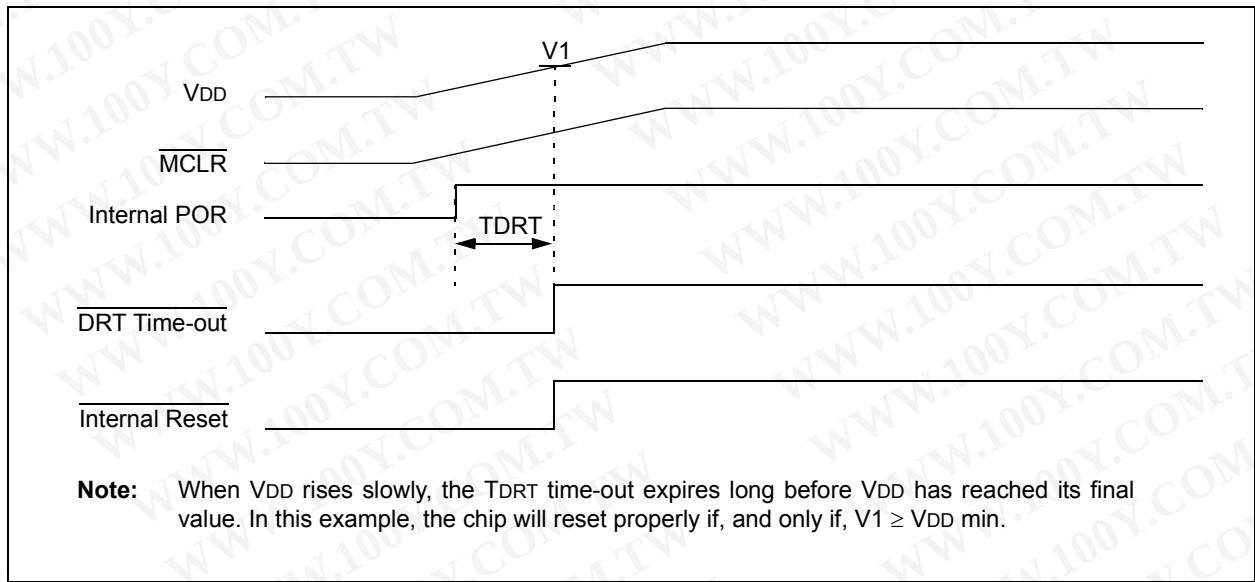
FIGURE 9-5: TIME-OUT SEQUENCE ON POWER-UP (MCLR TIED TO VDD): SLOW VDD RISE TIME
