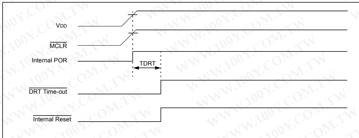
FIGURE 9-4: TIME-OUT SEQUENCE ON POWER-UP ( \overline{MCLR} TIED TO V_{DD} ): FAST V_{DD} RISE TIME
