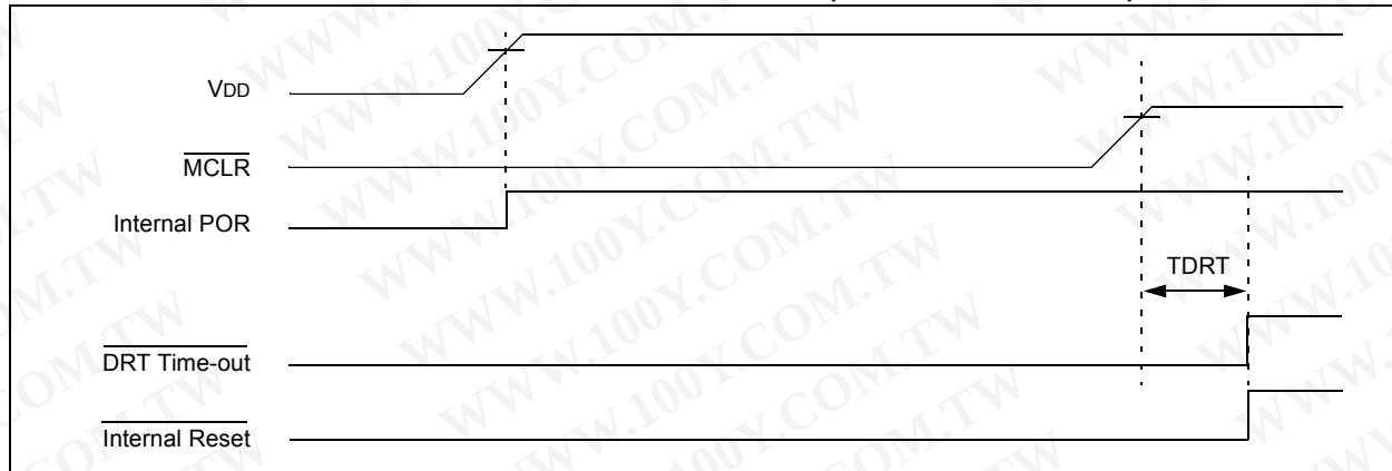
FIGURE 9-3: TIME-OUT SEQUENCE ON POWER-UP ( \overline{MCLR} PULLED LOW)
