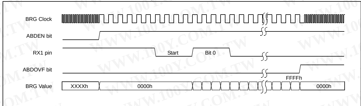
FIGURE 16-2: BRG OVERFLOW SEQUENCE
