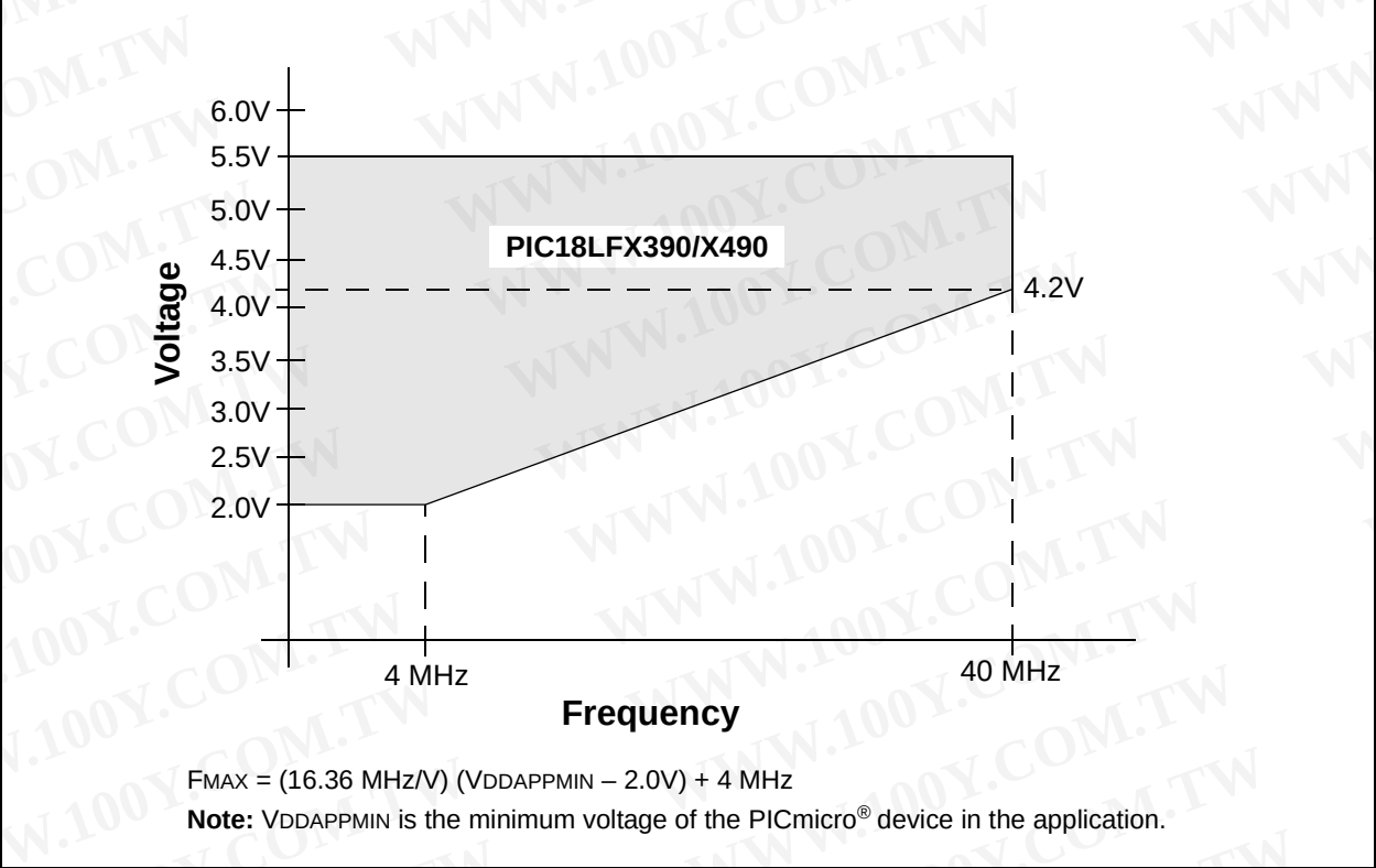
FIGURE 26-2: PIC18LF6390/6490/8390/8490 VOLTAGE-FREQUENCY GRAPH (INDUSTRIAL)
