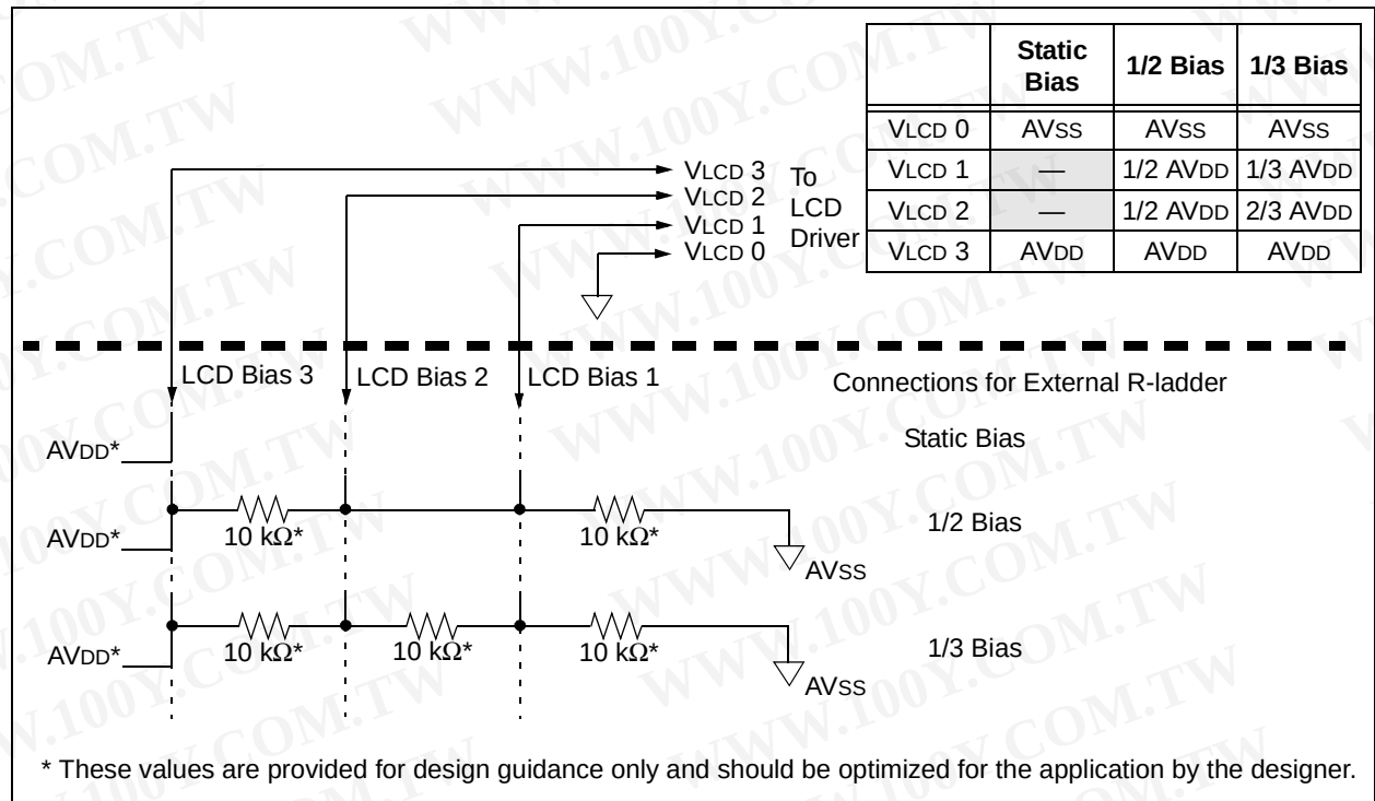
FIGURE 22-3: LCD BIAS RESISTOR LADDER CONNECTION DIAGRAM
