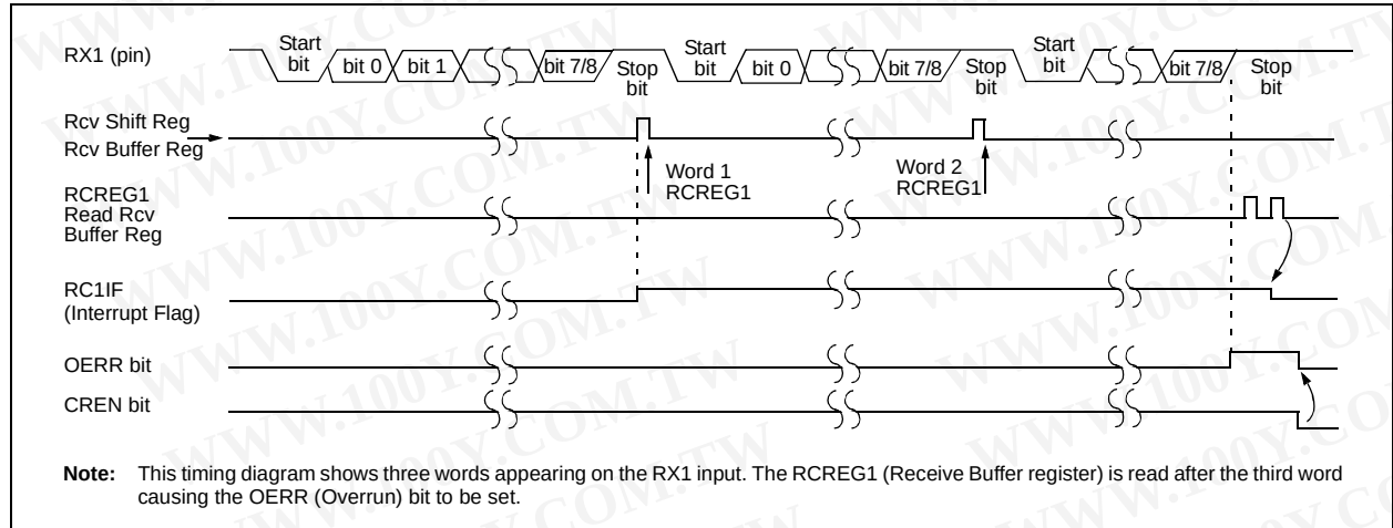
FIGURE 16-7: ASYNCHRONOUS RECEPTION
