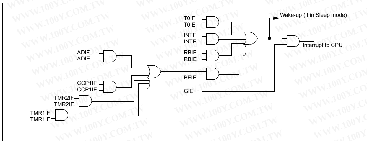
FIGURE 9-13: INTERRUPT LOGIC
