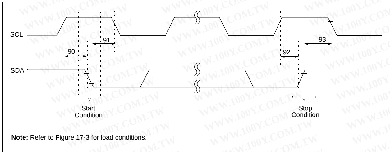
FIGURE 17-15: I 2 C BUS START/STOP BITS TIMING
