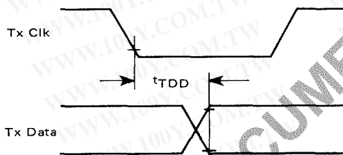
FIGURE 3 — TRANSMIT DATA OUTPUT DELAY
