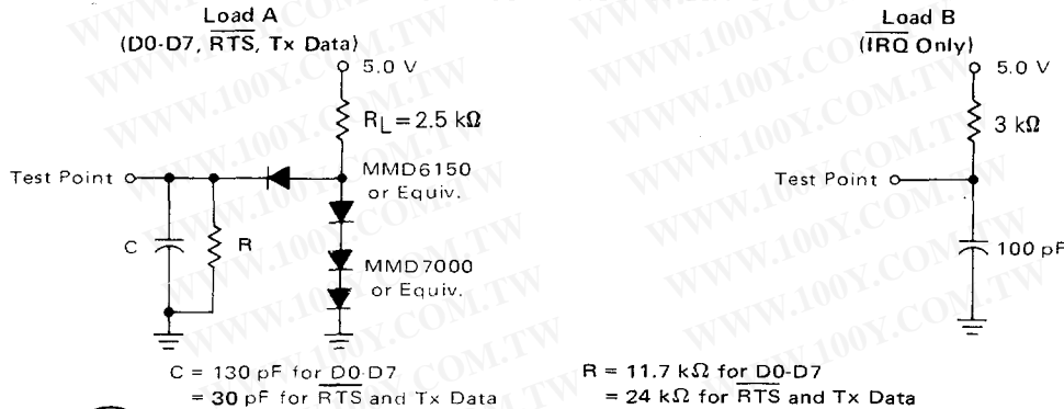
FIGURE 8 — BUS TIMING TEST LOADS
