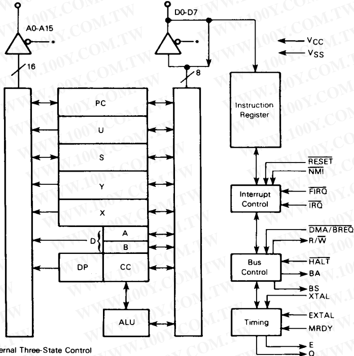
FIGURE 2 — MC6809 EXPANDED BLOCK DIAGRAM
