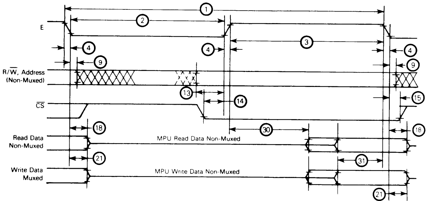
FIGURE 1 — BUS TIMING
