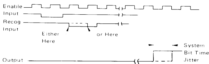
FIGURE 9 — INPUT JITTER
