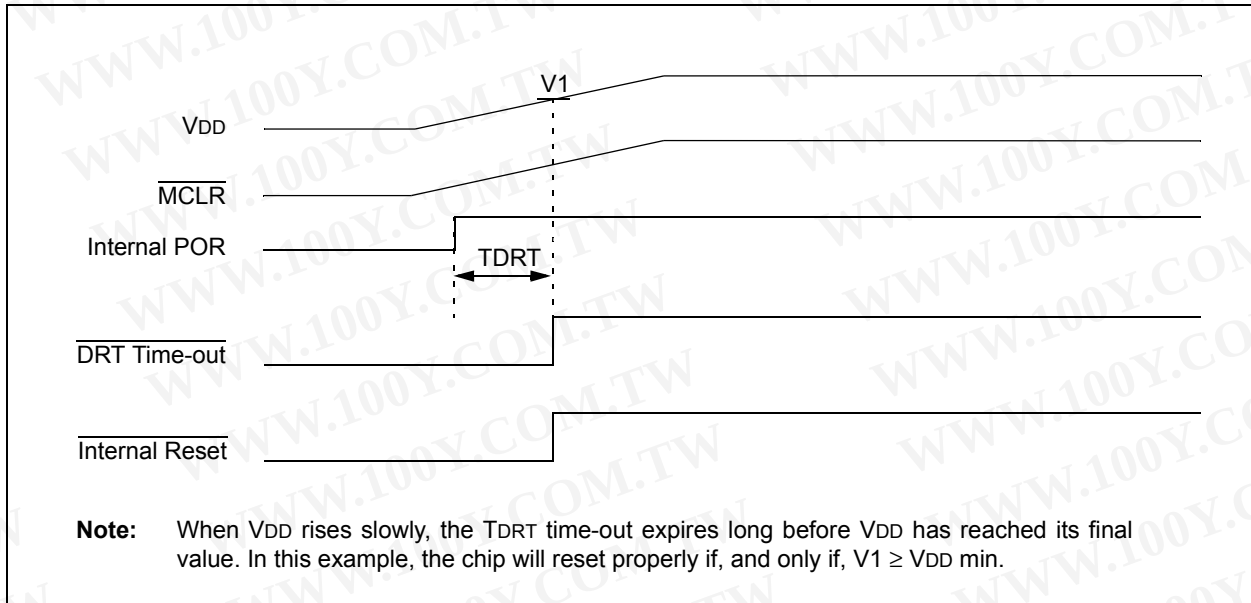
FIGURE 10-10: TIME-OUT SEQUENCE ON POWER-UP (MCLR TIED TO V DD ): SLOW V DD RISE TIME
