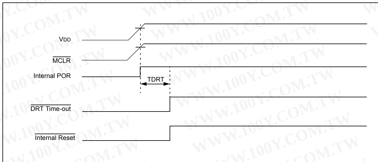
FIGURE 10-9: TIME-OUT SEQUENCE ON POWER-UP (MCLR TIED TO VDD): FAST VDD RISE TIME
