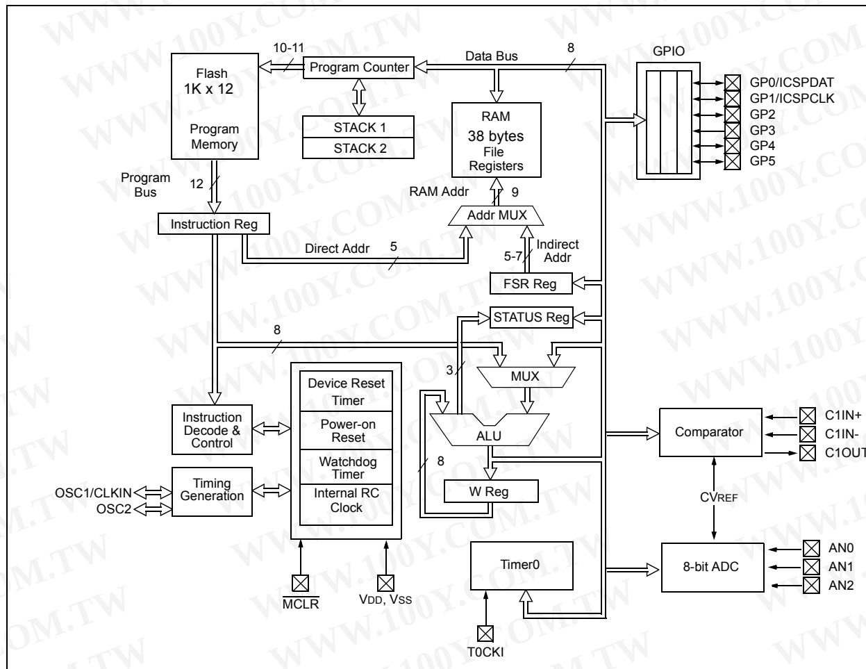
FIGURE 3-1: PIC12F510 SERIES BLOCK DIAGRAM
