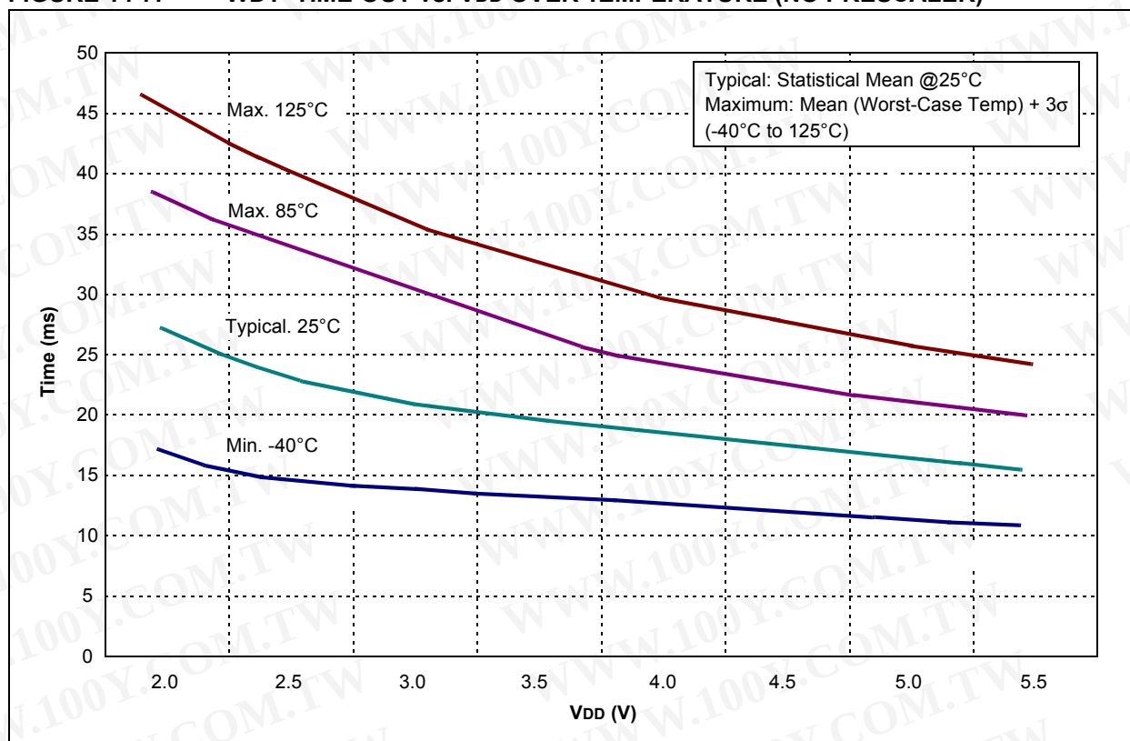
FIGURE 14-7: WDT TIME-OUT vs. VDD OVER TEMPERATURE (NO PRESCALER)
