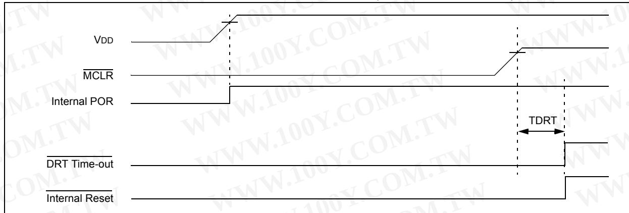
FIGURE 10-8: TIME-OUT SEQUENCE ON POWER-UP (MCLR PULLED LOW)
