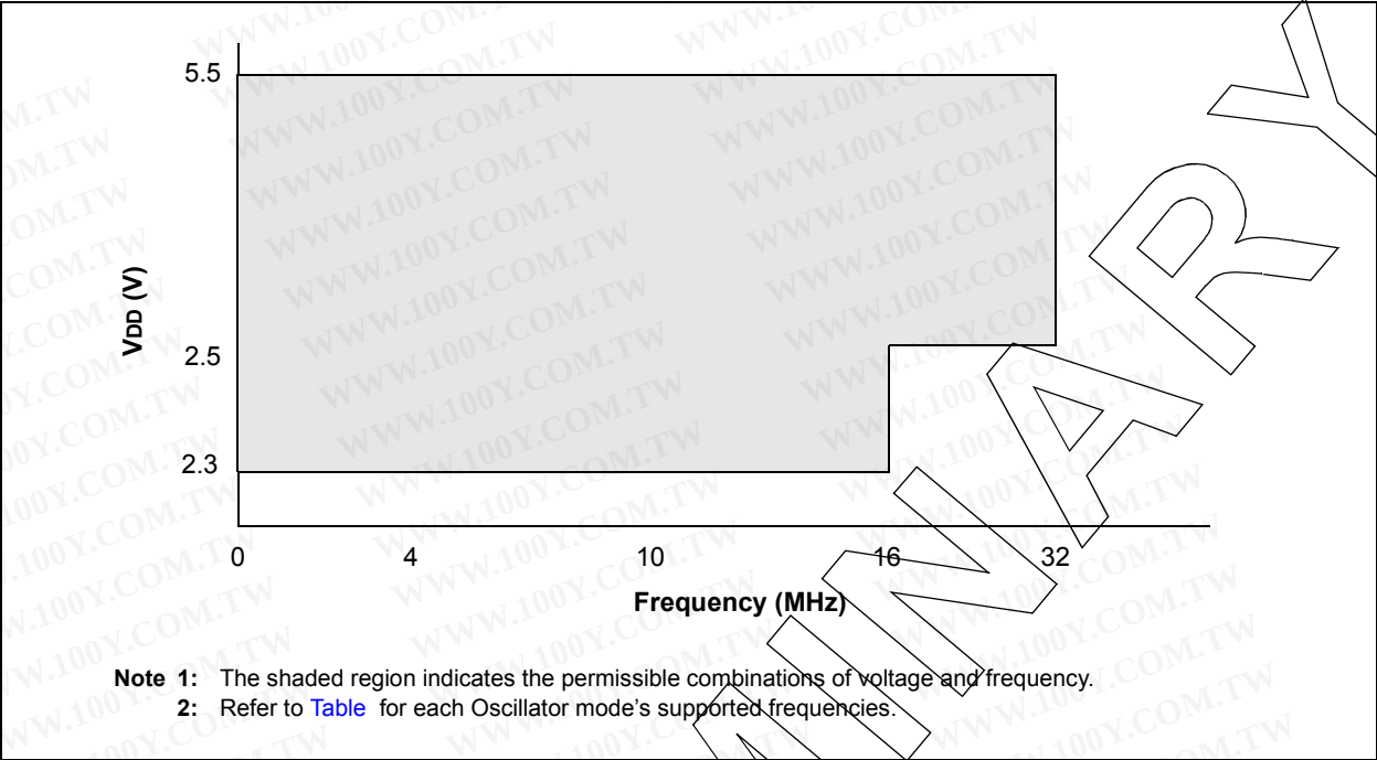
FIGURE 37-1: VOLTAGE FREQUENCY GRAPH, -40°C ≤ TA ≤ +125°C, PIC16F18854 ONLY
