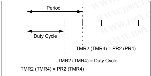
FIGURE 17-5: PWM OUTPUT
