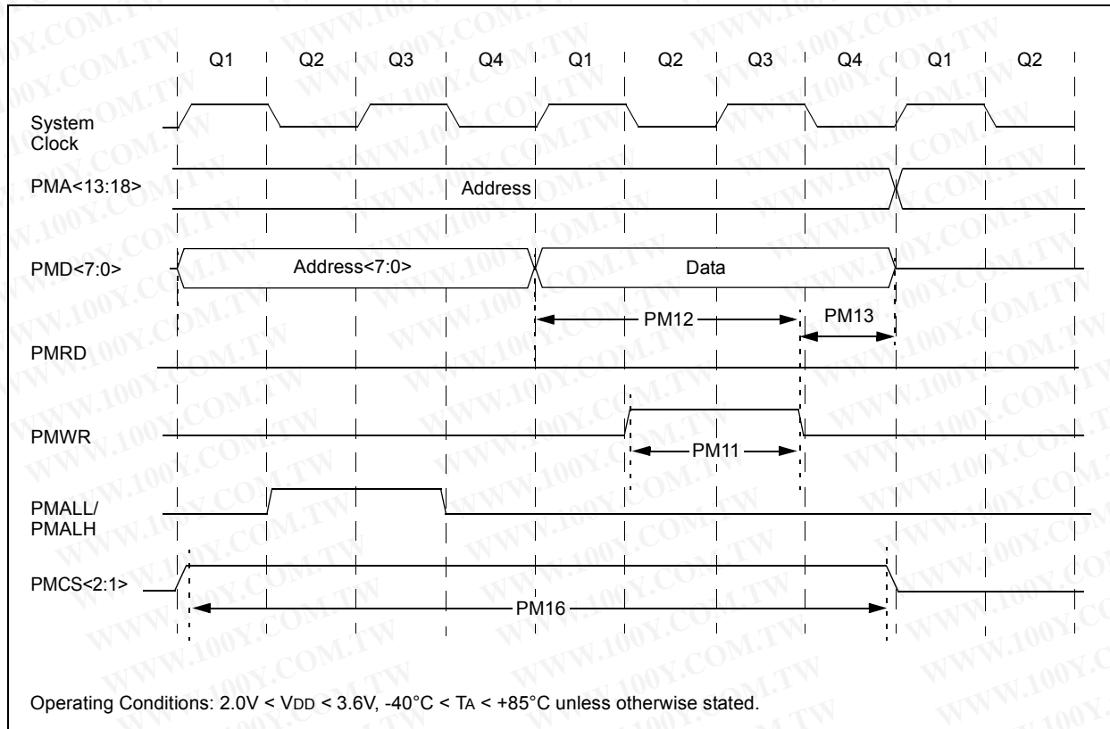
FIGURE 28-12: PARALLEL MASTER PORT WRITE TIMING DIAGRAM
