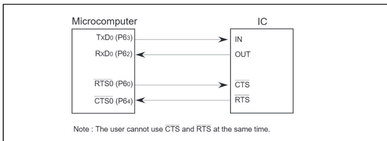
Figure 1.19.19. The separate \overline{\text{CTS}} / \overline{\text{RTS}} pins function usage
