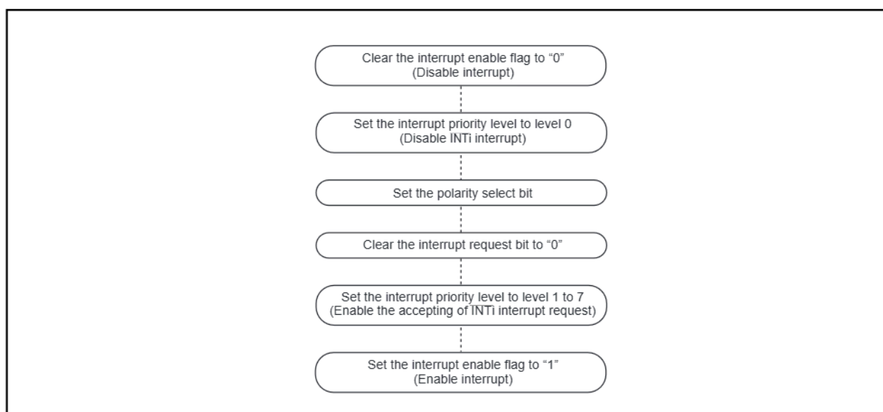
Figure 1.14.13. Switching condition of \overline{\text{INT}} interrupt request
