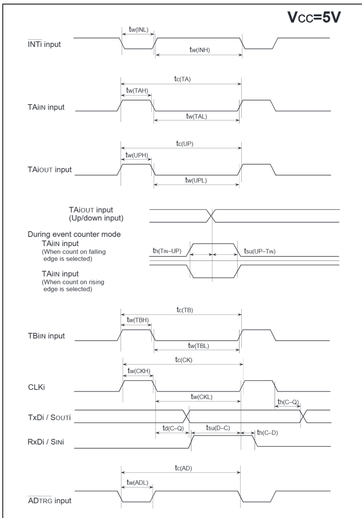
Figure 1.26.2. Timing
