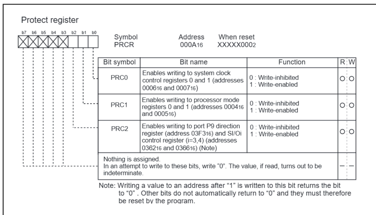
Figure 1.13.6. Protect register
