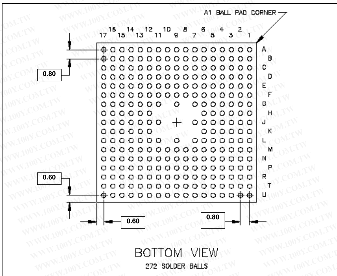
Figure 25-2. 272-FBGA-1414 Package Dimension 2
