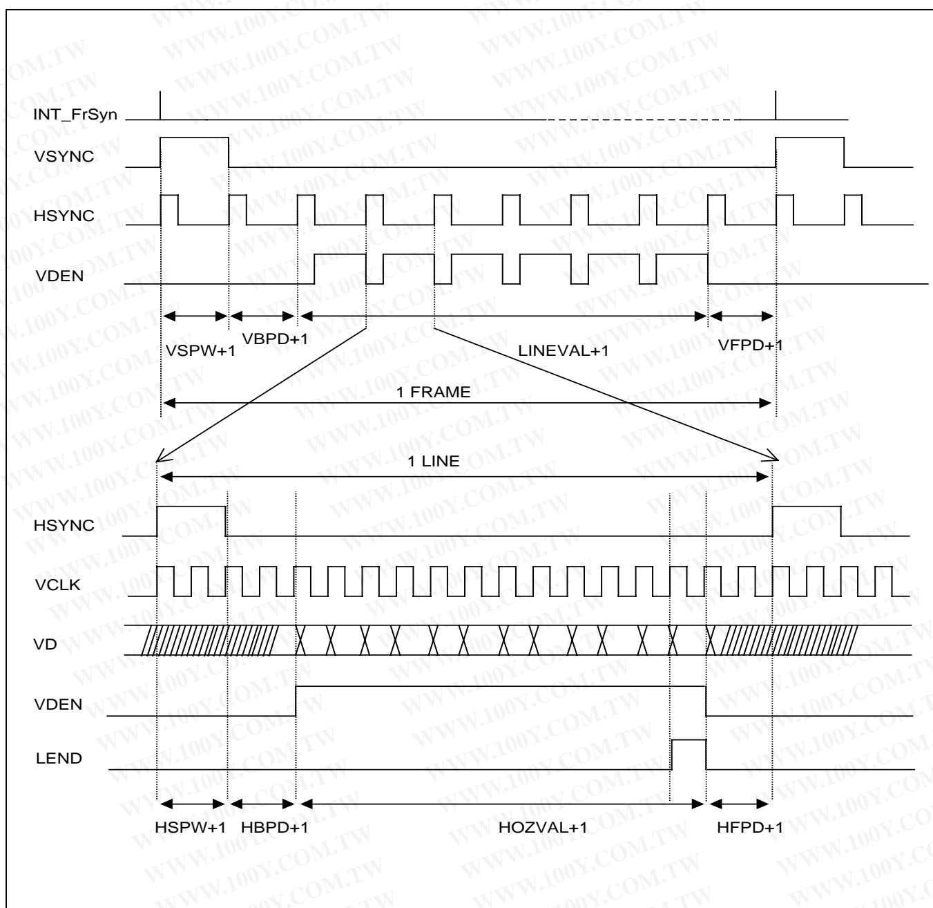
Figure 15-6. TFT LCD Timing Example
