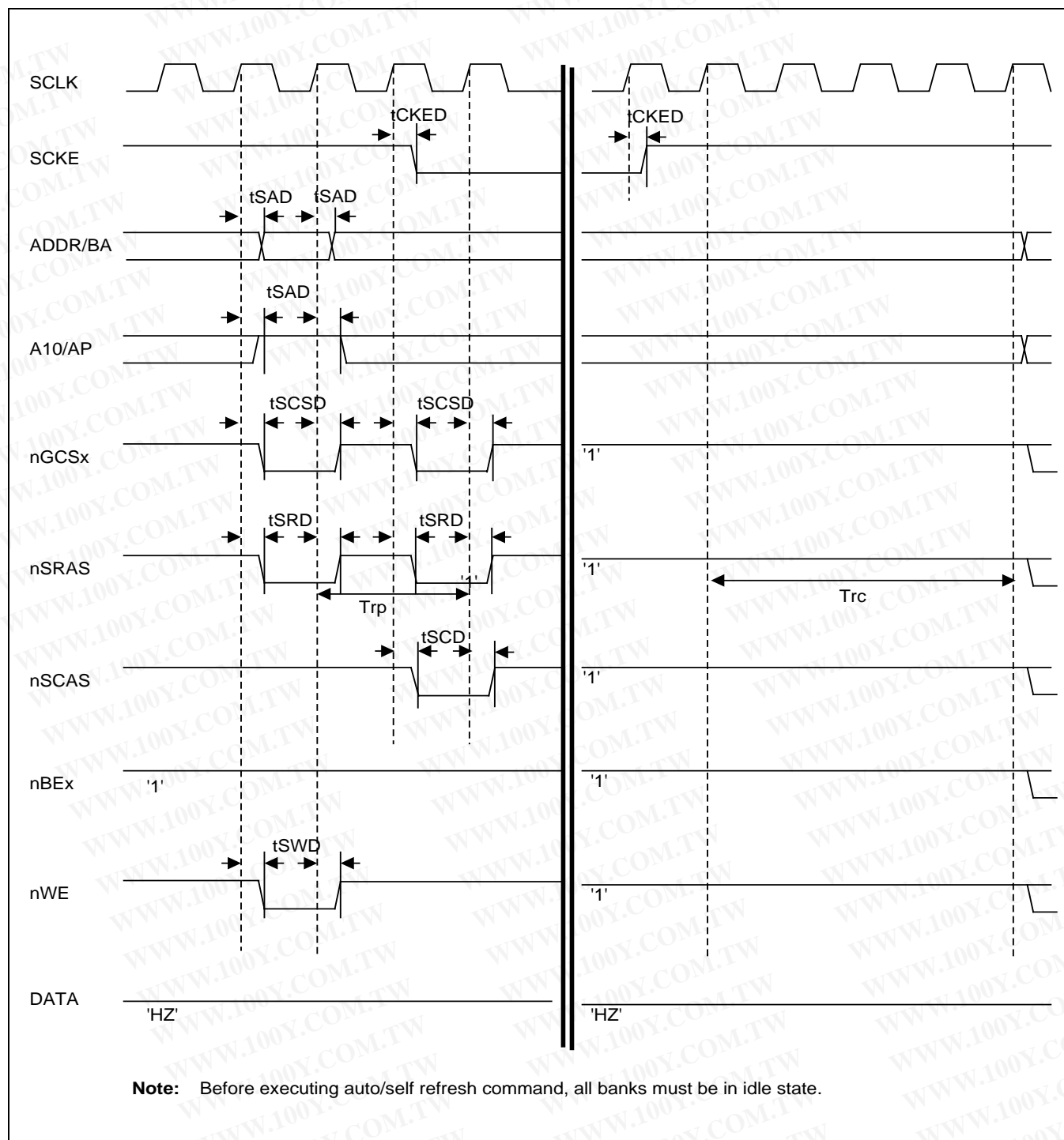
Figure 24-19. SDRAM Self Refresh Timing (Trp=2, Trc=4)
