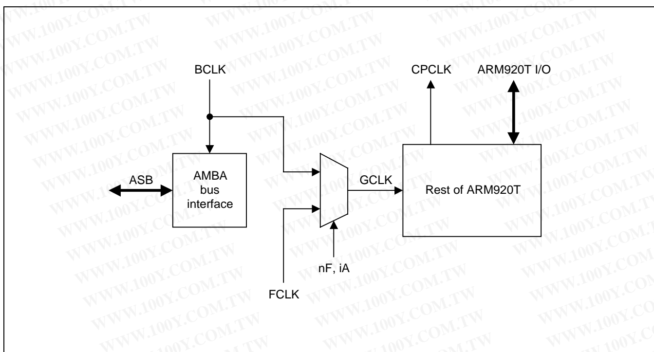
Figure 5-1. ARM920T Clocking
