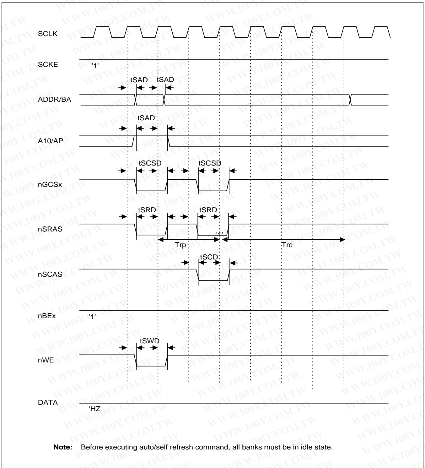
Figure 24-17. SDRAM Auto Refresh Timing (Trp=2, Trc=4)
