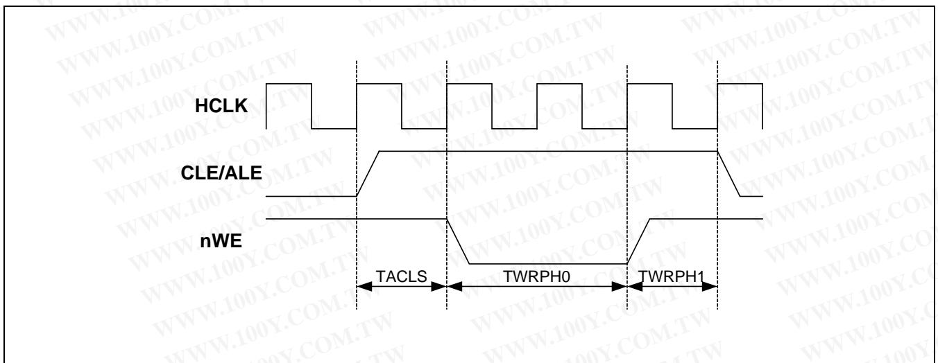
Figure 6-3. TACLS=0, TWRPH0=1, TWRPH1=0
