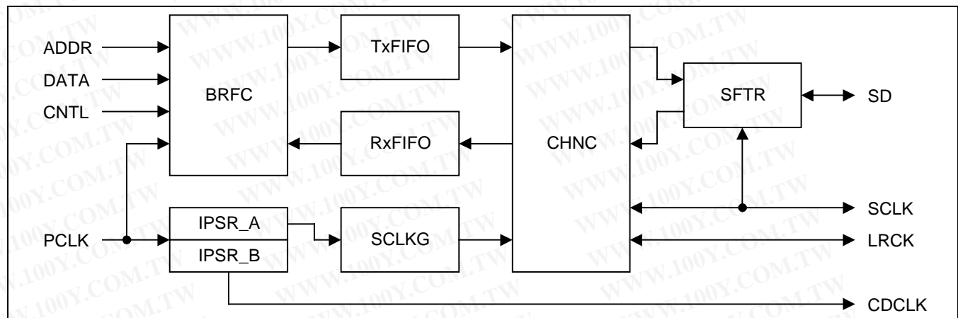
Figure 21-1. IIS-Bus Block Diagram
