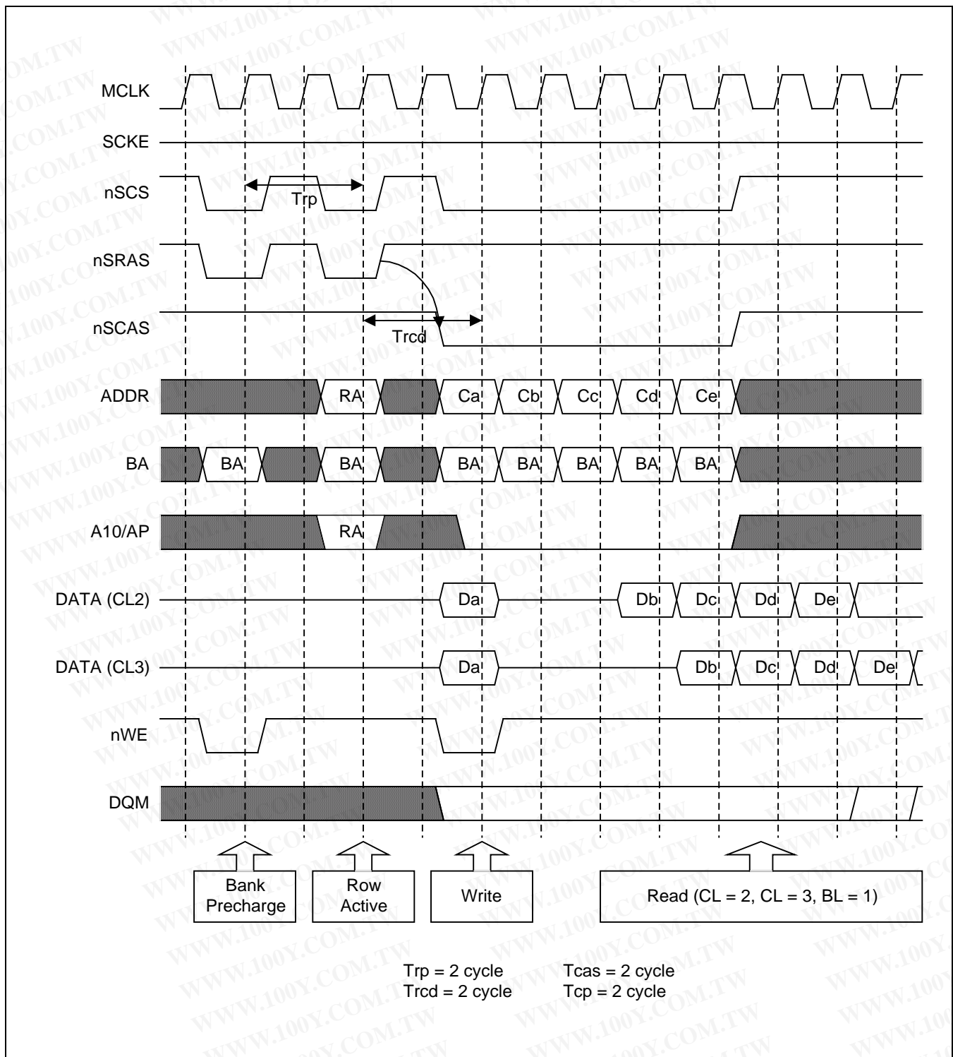
Figure 5-13. S3C2410X01 SDRAM Timing Diagram
