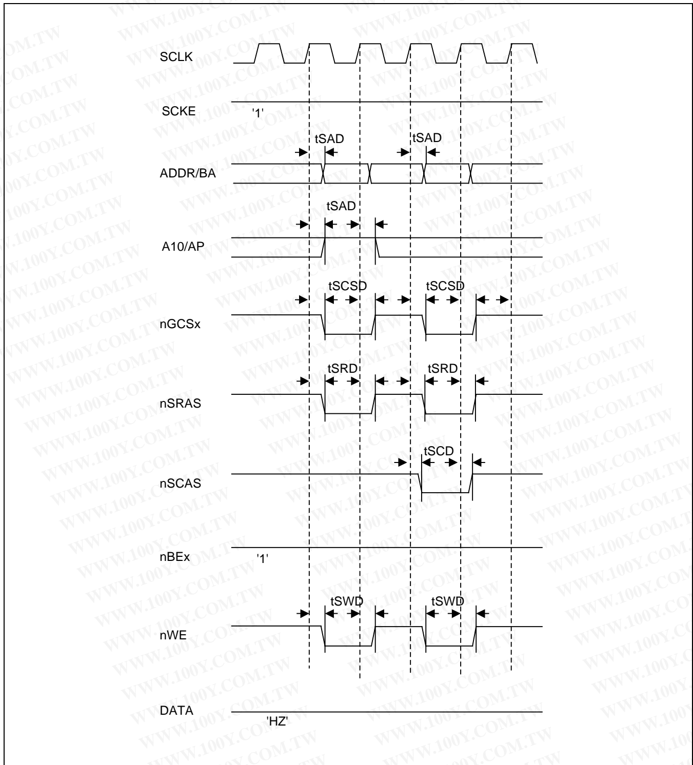
Figure 24-14. SDRAM MRS Timing
