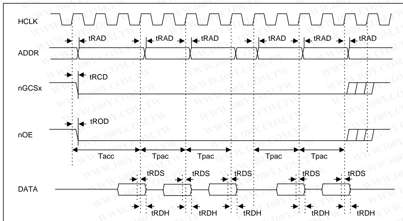
Figure 24-12. Masked-ROM Consecutive READ Timing ( T_{acs}=0 , T_{cos}=0 , T_{acc}=3 , T_{pac}=2 , PMC=01/10/11 )
