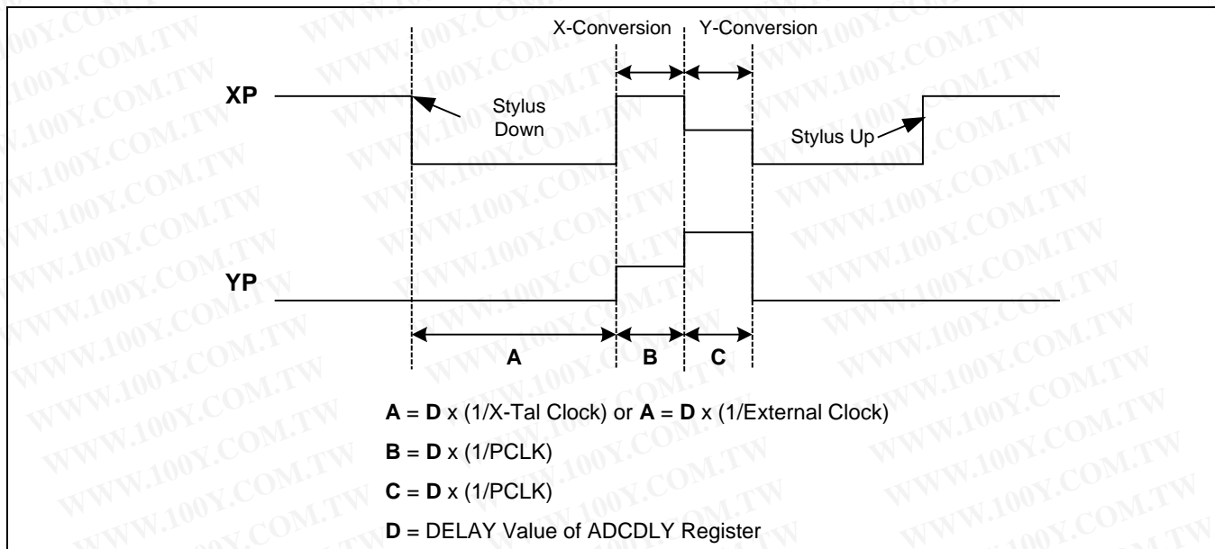
Figure 16-3 Timing Diagram in Auto (Sequential) X/Y Position Conversion Mode
