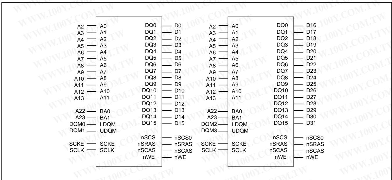
Figure 5-11. Memory Interface with 16-bit SDRAM (4Mx16 * 2ea, 4banks)
