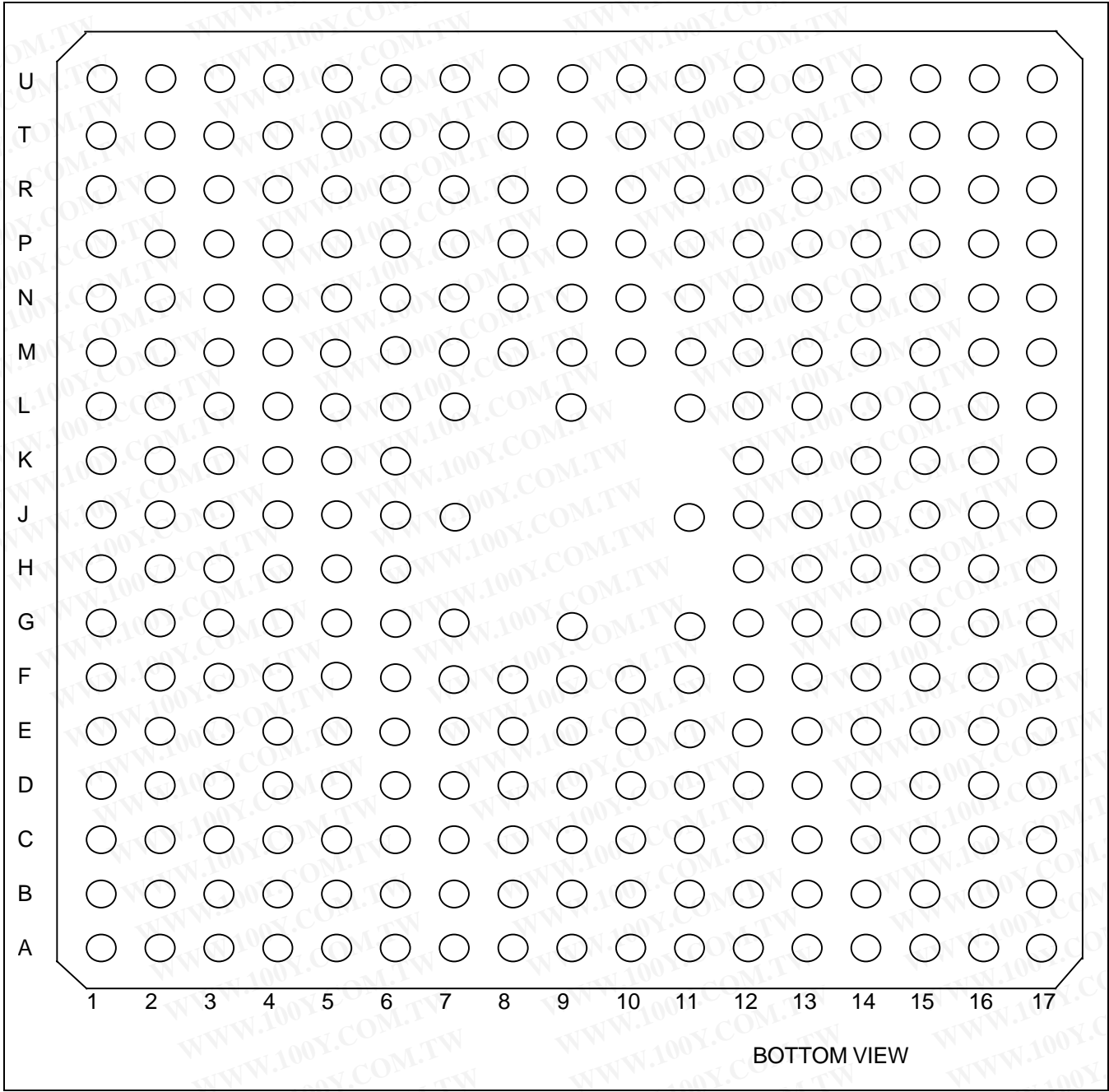
Figure 1-3. S3C2410X01 Pin Assignments (272 FBGA)
