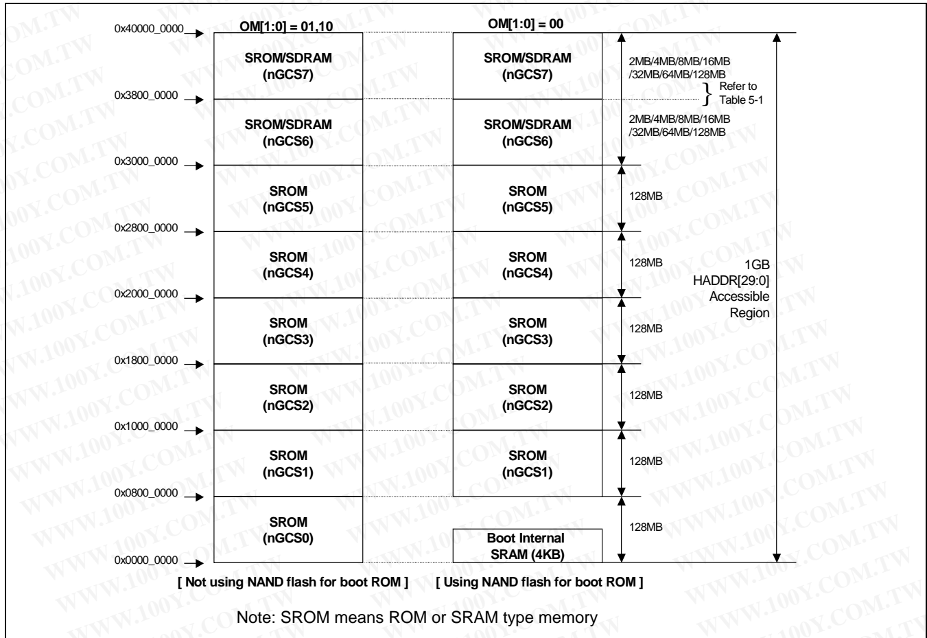
Figure 5-1. S3C2410X01 Memory Map after Reset
