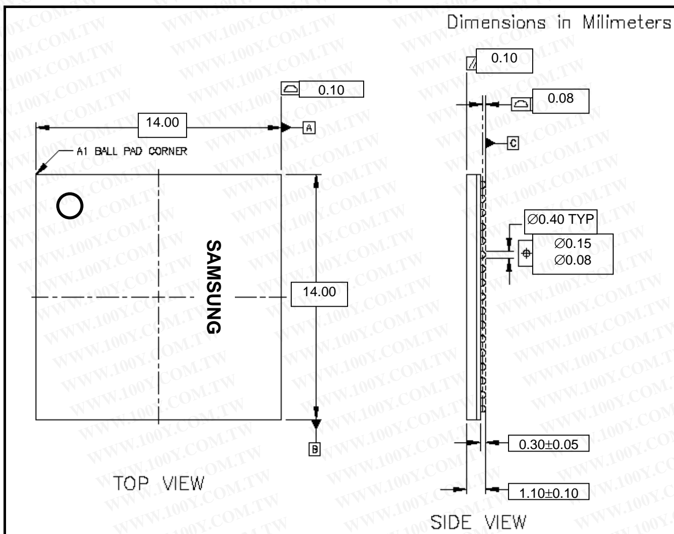
Figure 25-1. 272-FBGA-1414 Package Dimension 1
