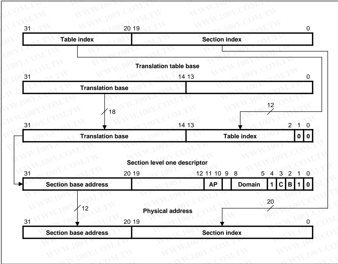
Figure 3-5. Section Translation
