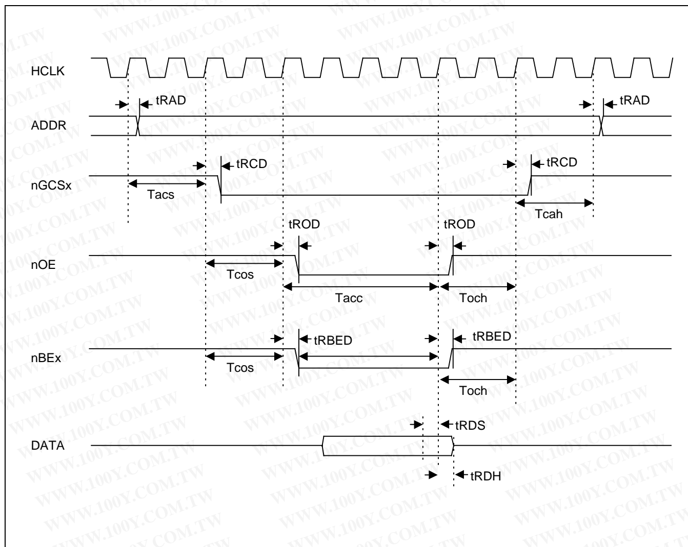
Figure 24-8. ROM/SRAM READ Timing (II) (Tacs=2, Tcos=2, Tacc=4, Toch=2, Tcah=2cycle, PMC=0, ST=1)
