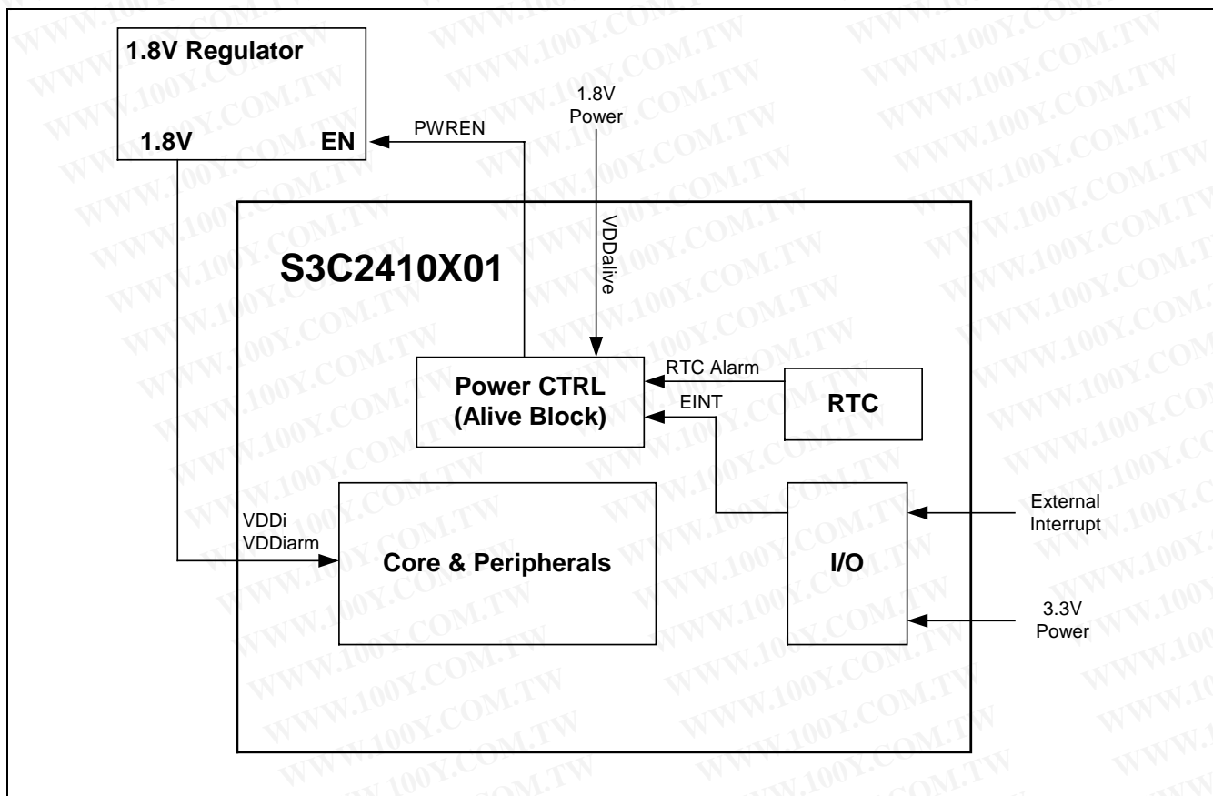
Figure 7-14. Power-OFF Mode
