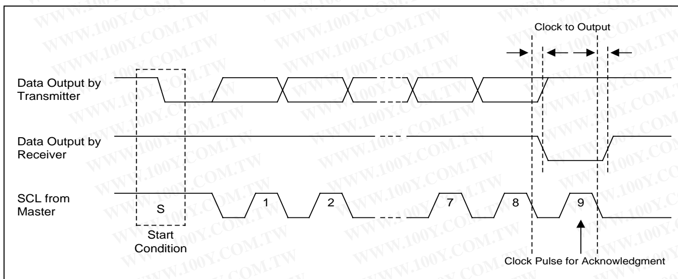
Figure 20-5. Acknowledge on the IIC-Bus
