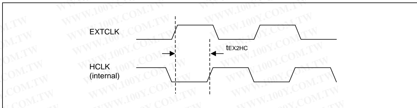
Figure 24-3. EXTCLK/HCLK in case that EXTCLK is used without the PLL
