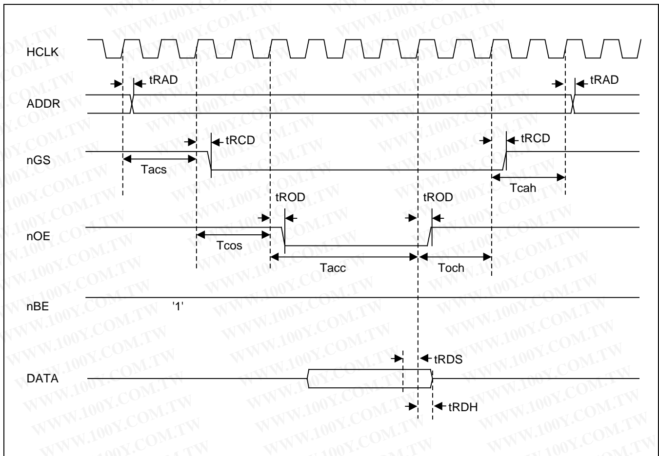
Figure 24-7. ROM/SRAM READ Timing (I) (Tacs=2, Tcos=2, Tacc=4, Toch=2, Tcah=2, PMC=0, ST=0)
