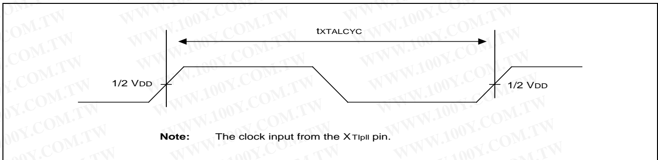
Figure 24-1. XTlpll Clock Timing
