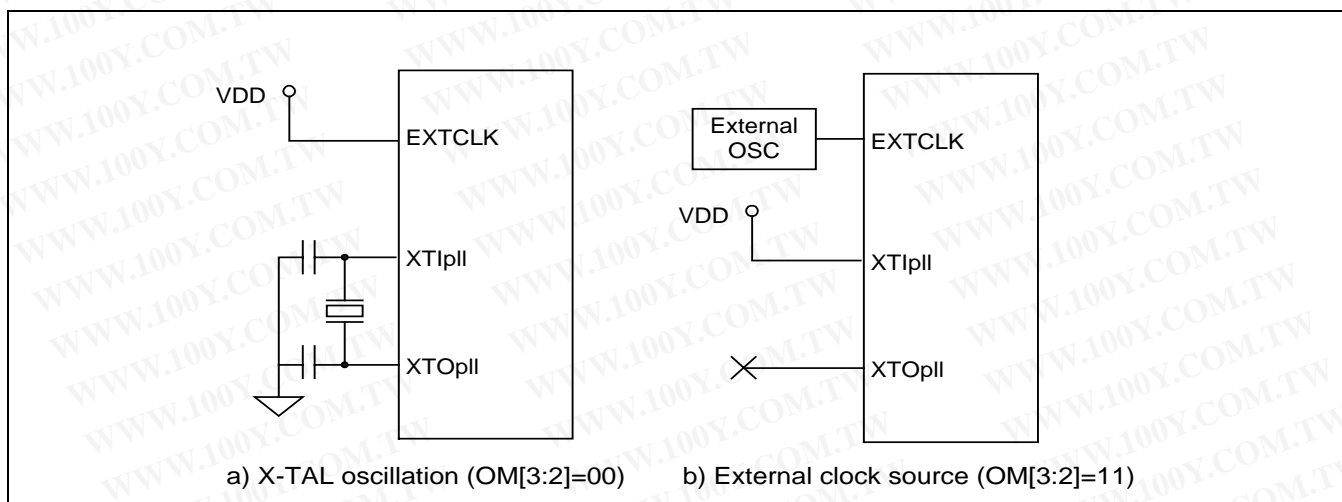
Figure 7-3. Main Oscillator Circuit Examples
