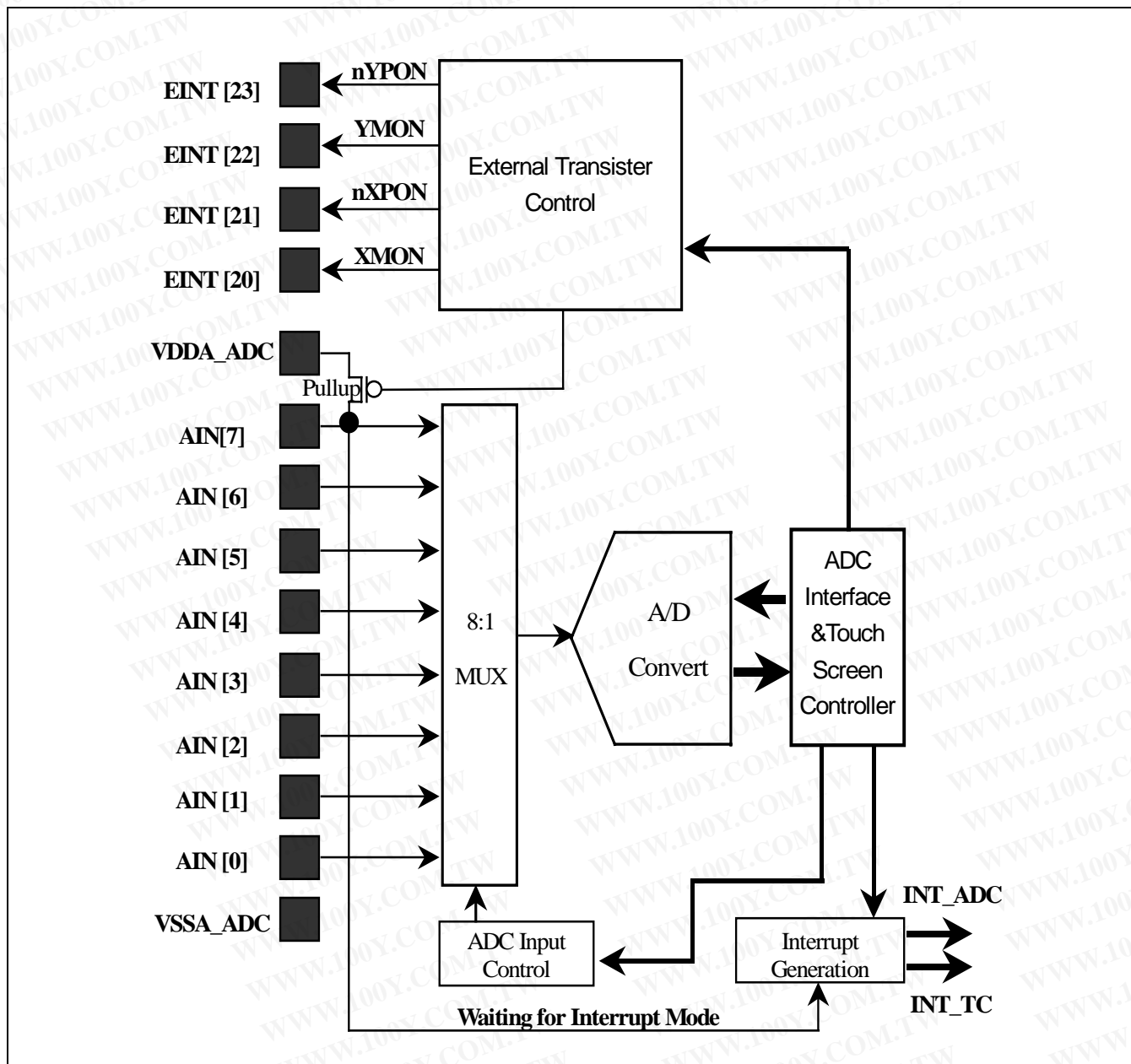
Figure 16-1. ADC and Touch Screen Interface Functional Block Diagram
