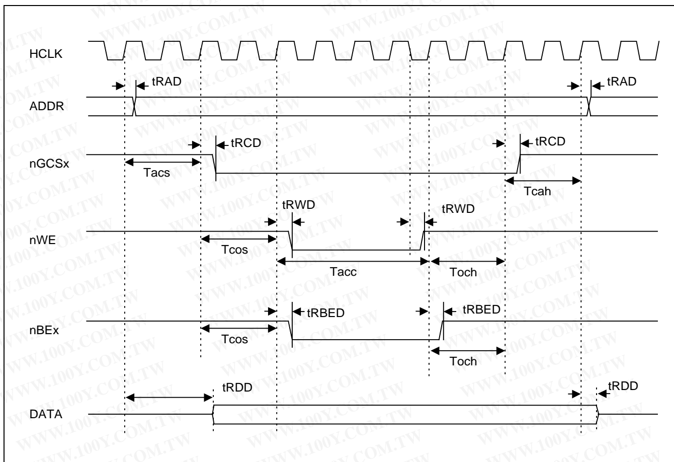
Figure 24-10. ROM/SRAM WRITE Timing (II) (Tacs=2, Tcos=2, Tacc=4, Toch=2, Tcah=2, PMC=0, ST=1)
