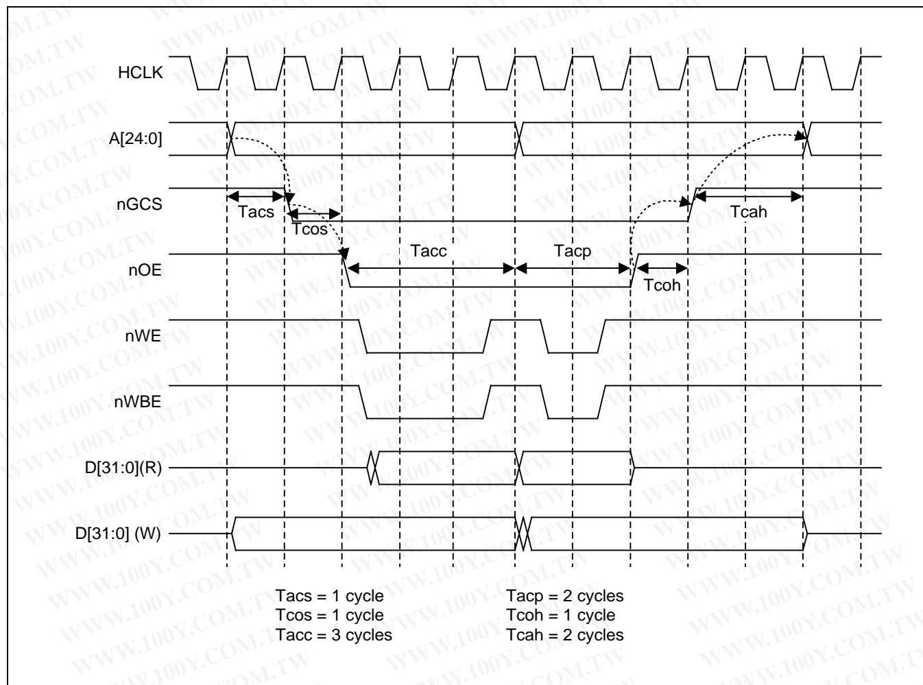
Figure 5-12. S3C2410X01 nGCS Timing Diagram
