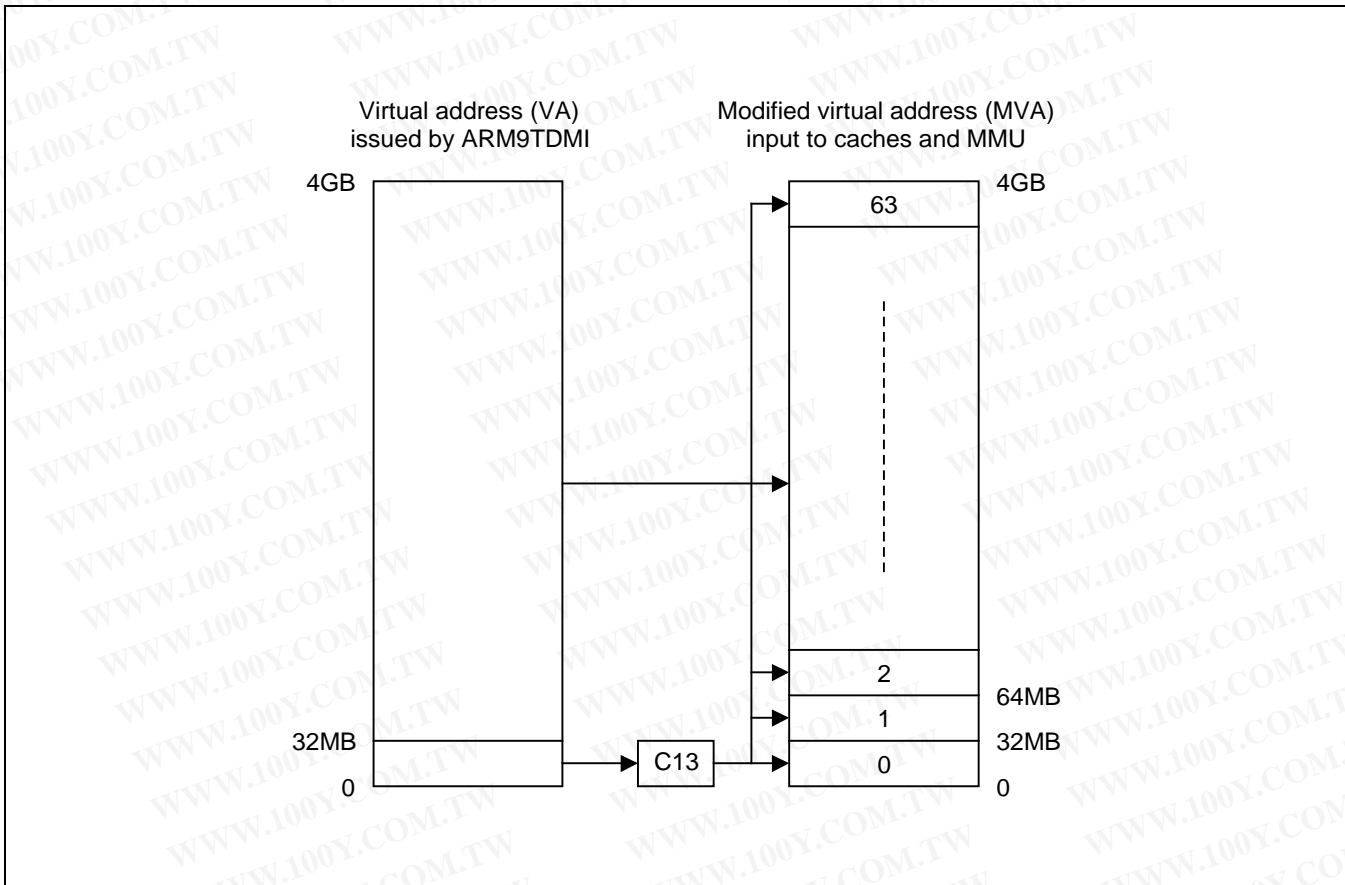
Figure 2-8. Address Mapping Using CP15 Register 13
