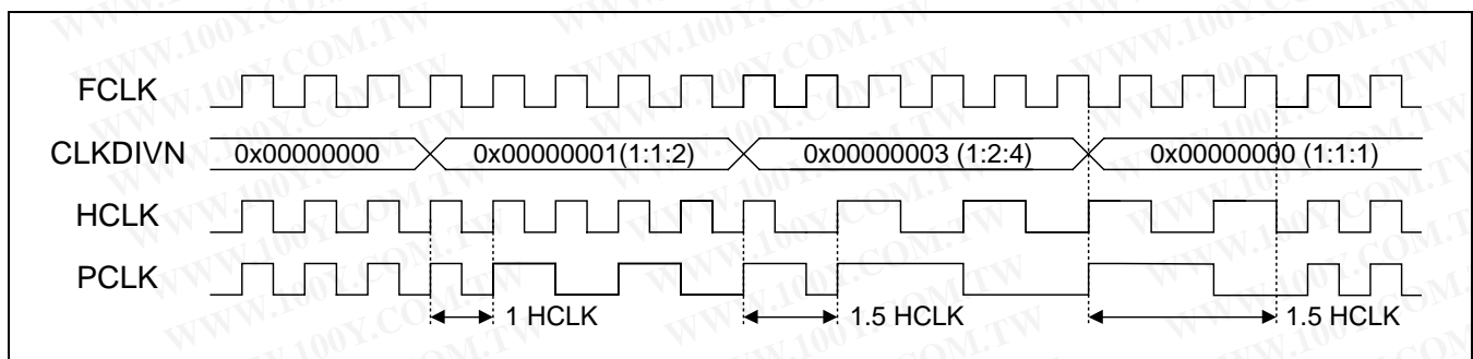
Figure 7-6. Changing CLKDIVN Register Value
