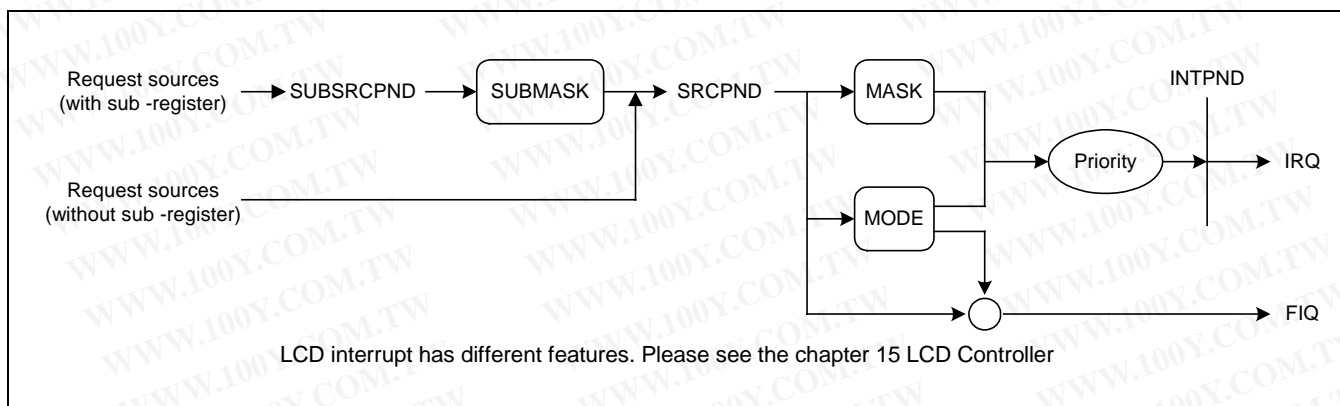
FIGURE 14-1. INTERRUPT PROCESS DIAGRAM
