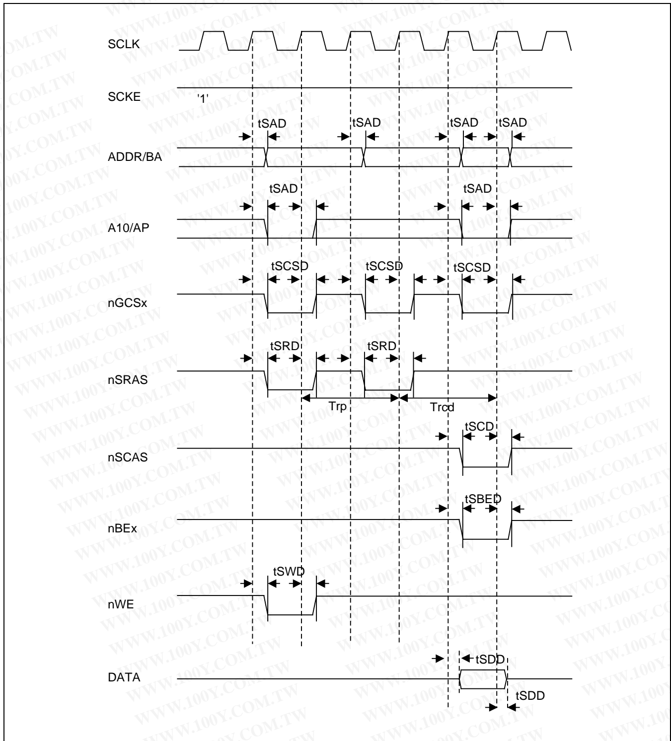
Figure 24-20. SDRAM Single Write Timing ( Trp=2 , Trcd=2 )
