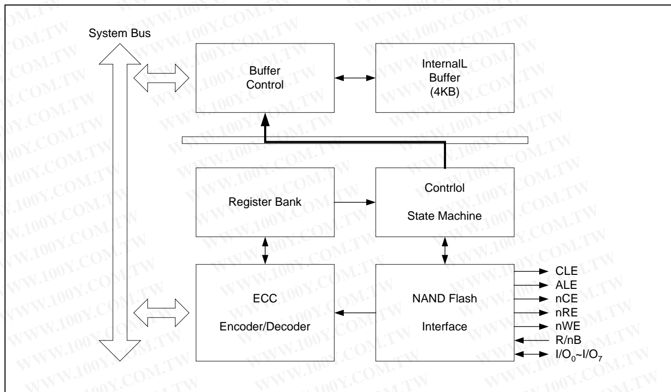
Figure 6-1. NAND Flash Controller Block Diagram
