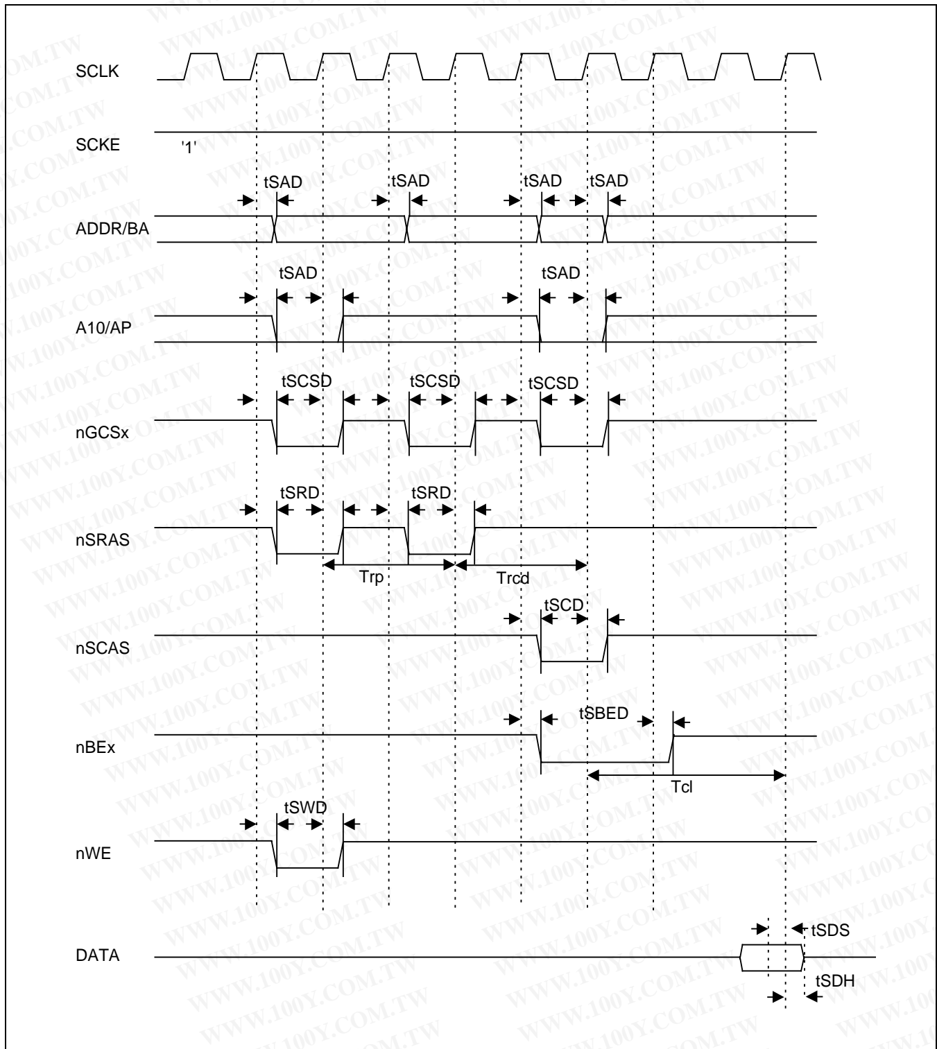
Figure 24-16. SDRAM Single READ Timing(II) ( T_{rp}=2 , T_{rcd}=2 , T_{cl}=3 )
