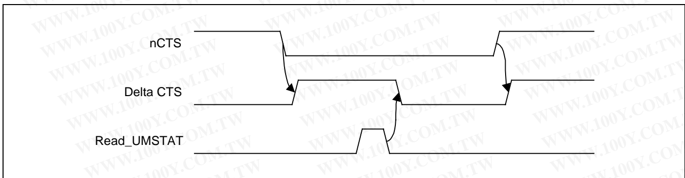
Figure 11-8. nCTS and Delta CTS Timing Diagram
