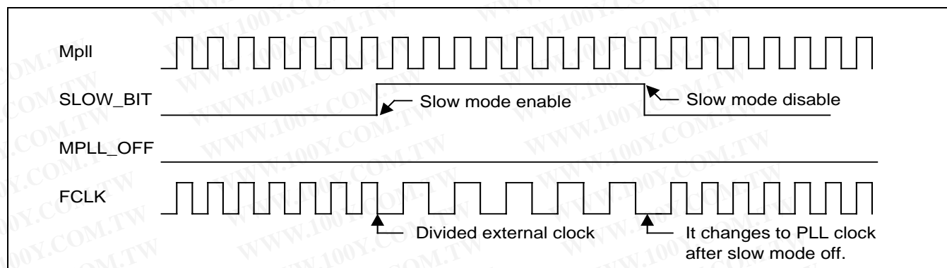
Figure 7-11. Issuing Exit_from_Slow_mode command in PLL on state
