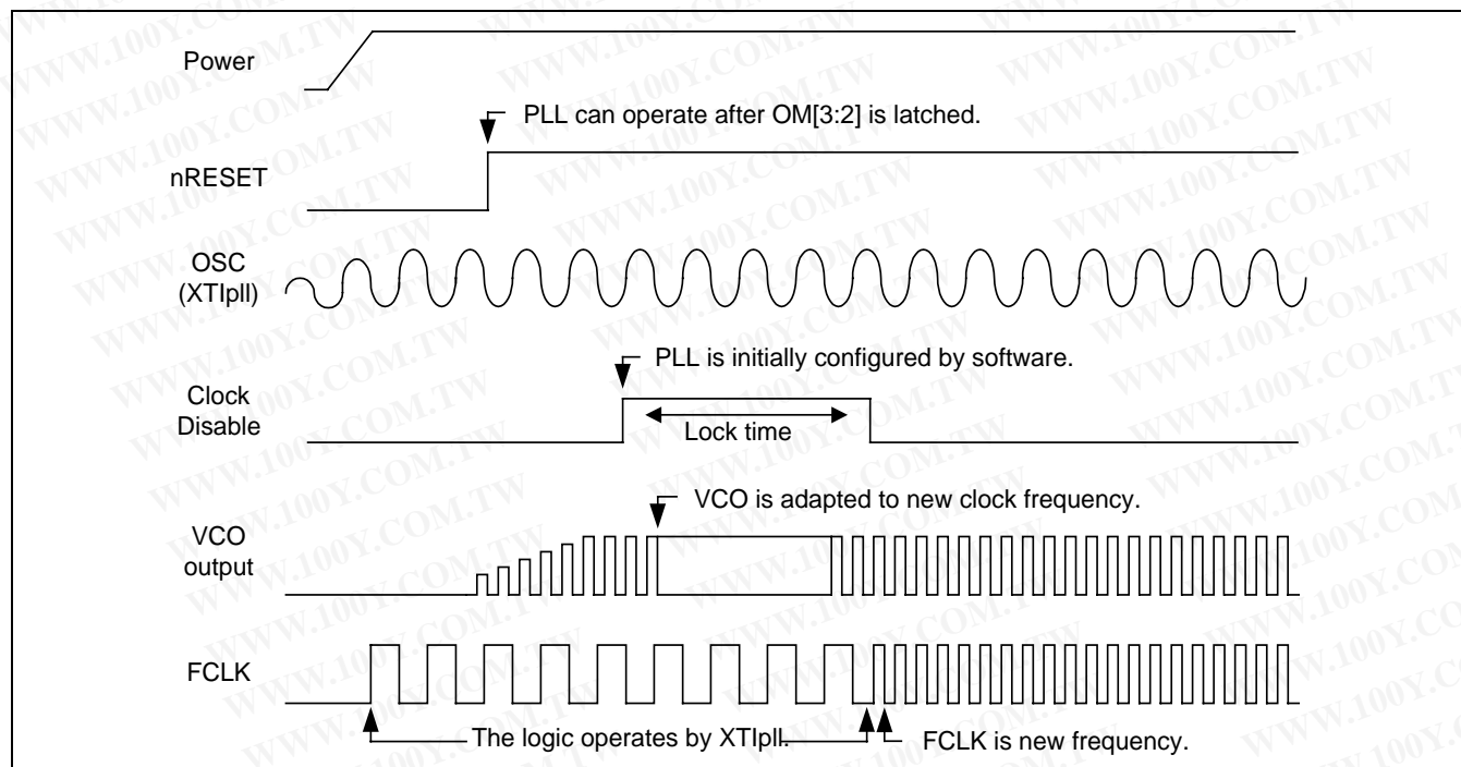
Figure 7-4. Power-On Reset Sequence (when the external clock source is a crystal oscillator)
