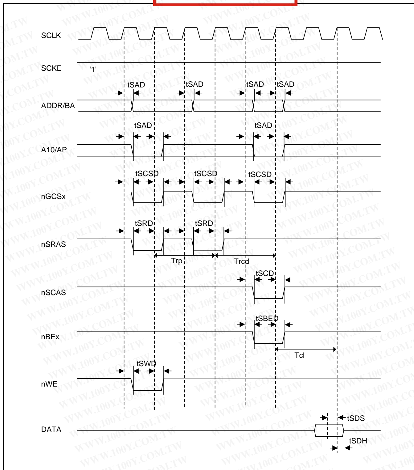
Figure 24-15. SDRAM Single READ Timing(I) (Trp=2, Trcd=2, Tcl=2)
