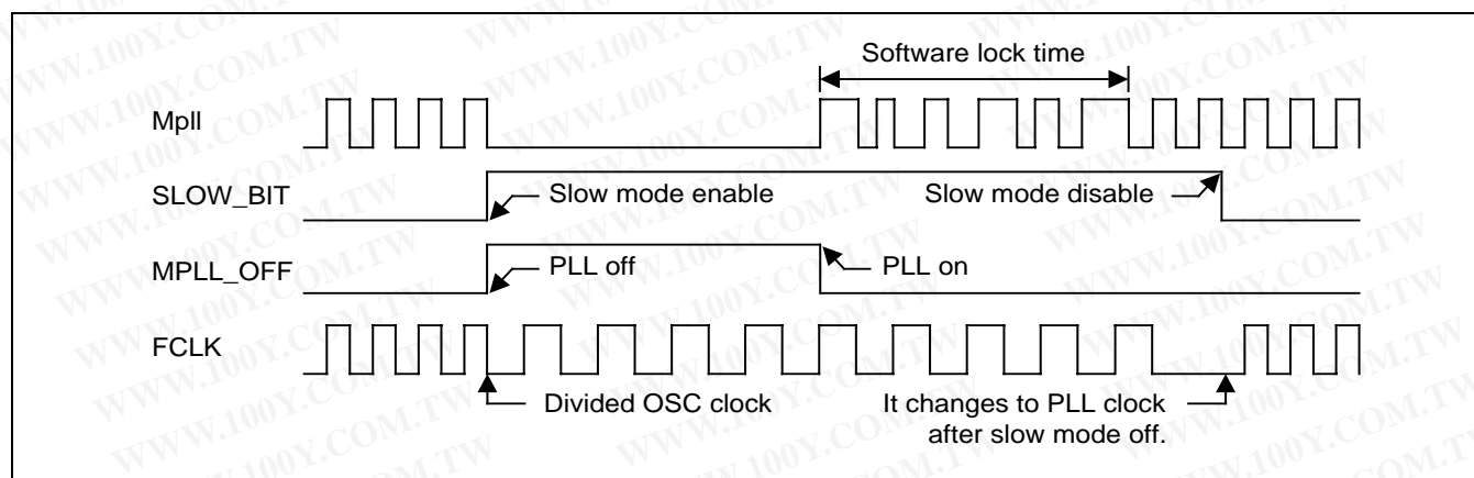
Figure 7-12. Issuing Exit_from_Slow_mode command after lock time
