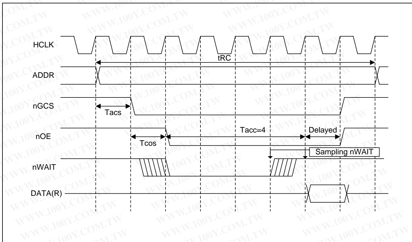
Figure 5-2. S3C2410X01 External nWAIT Timing Diagram ( T_{acc}=4 )
