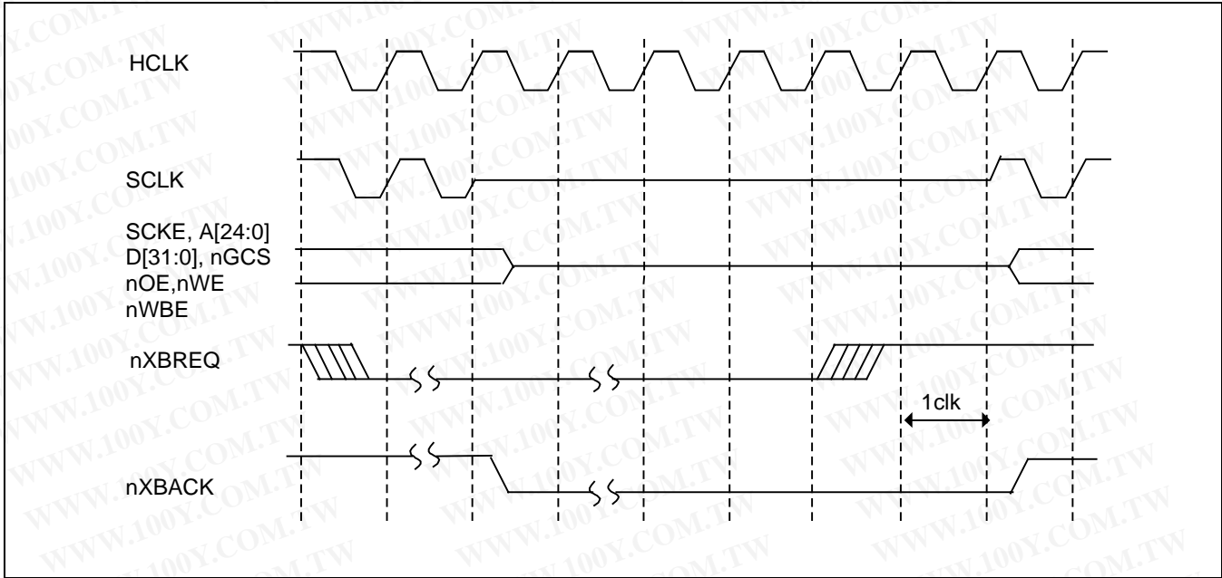
Figure 5-3. S3C2410X01 nXBREQ/nXBACK Timing Diagram
