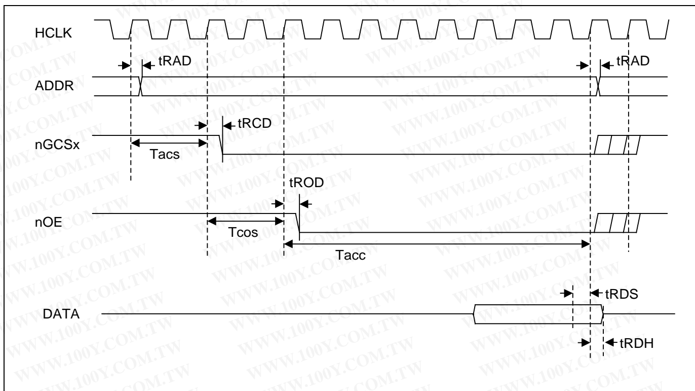
Figure 24-11. Masked-ROM Single READ Timing ( T_{acs}=2 , T_{cos}=2 , T_{acc}=8 , PMC=01/10/11 )
