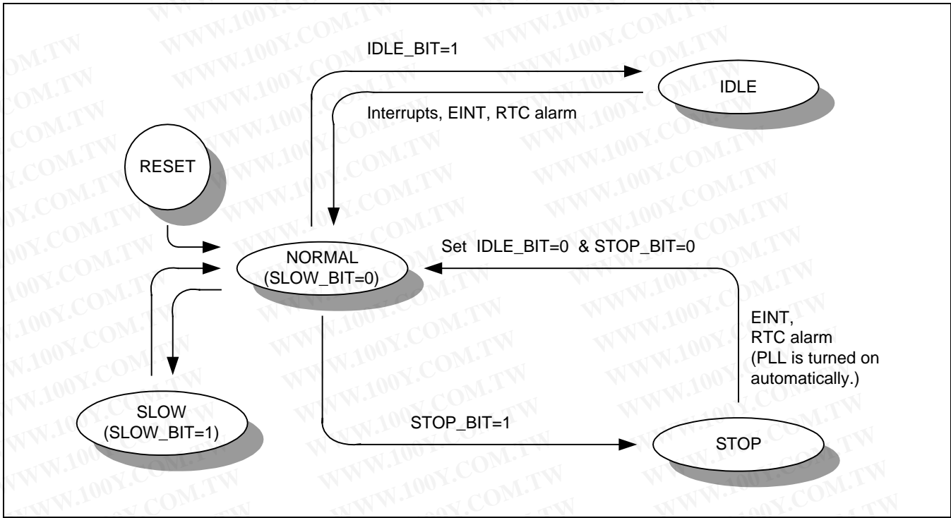
Figure 7-8. Power Management State Machine
