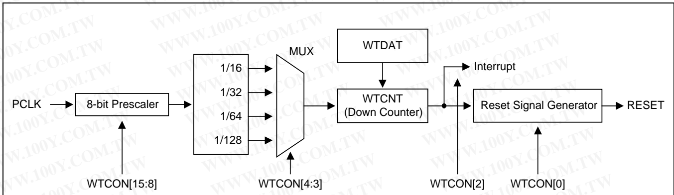
Figure 18-1. Watchdog Timer Block Diagram
