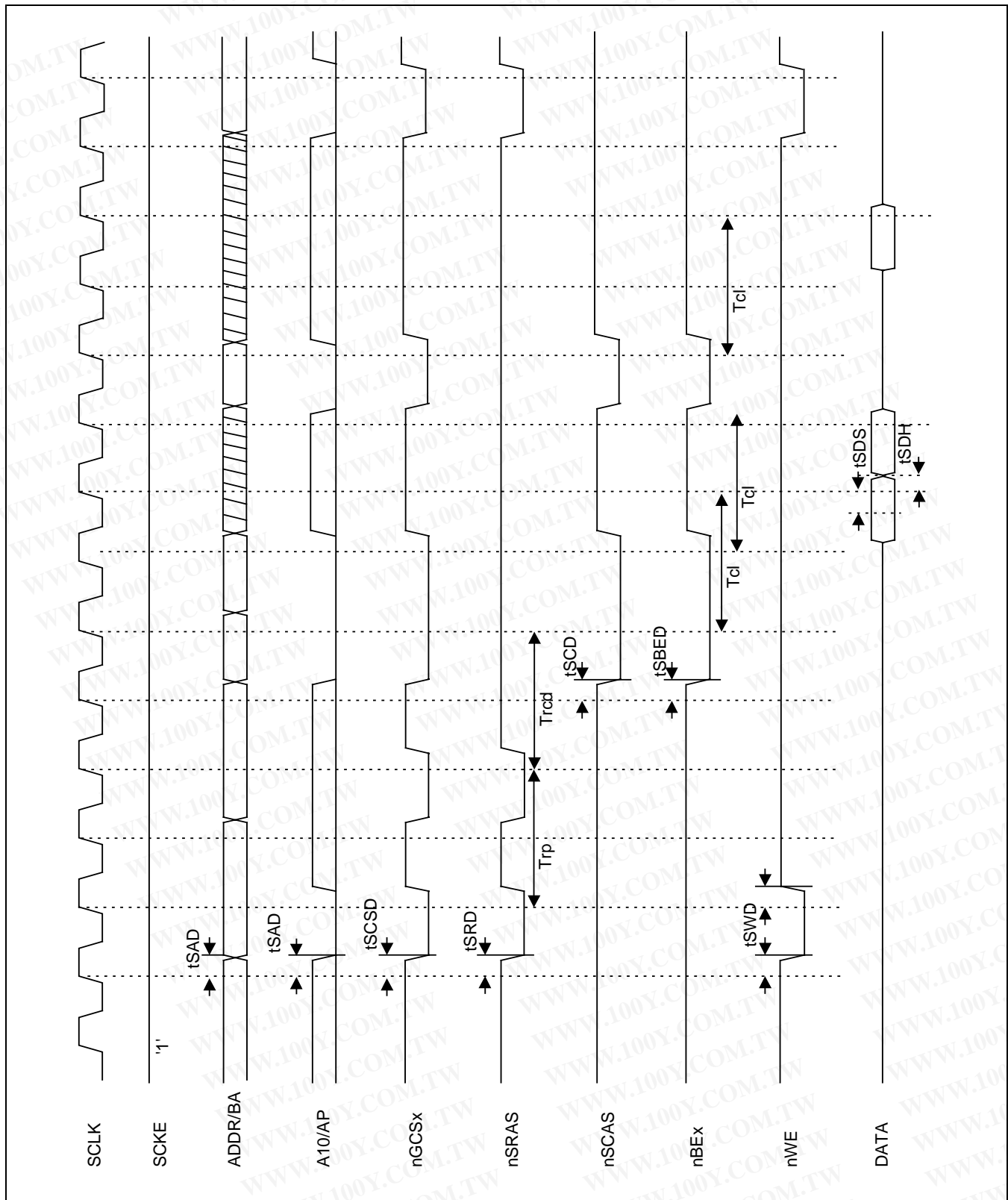
Figure 24-18. SDRAM Page Hit-Miss READ Timing ( Trp=2 , Trcd=2 , Tcl=2 )
