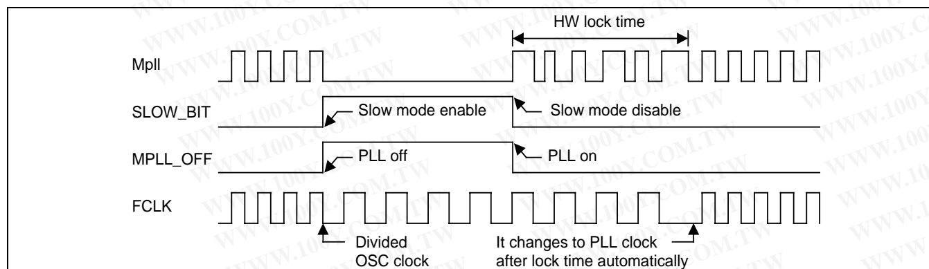
Figure 7-13. Issuing Exit_from_Slow_mode command and the instant PLL_on command simultaneously
