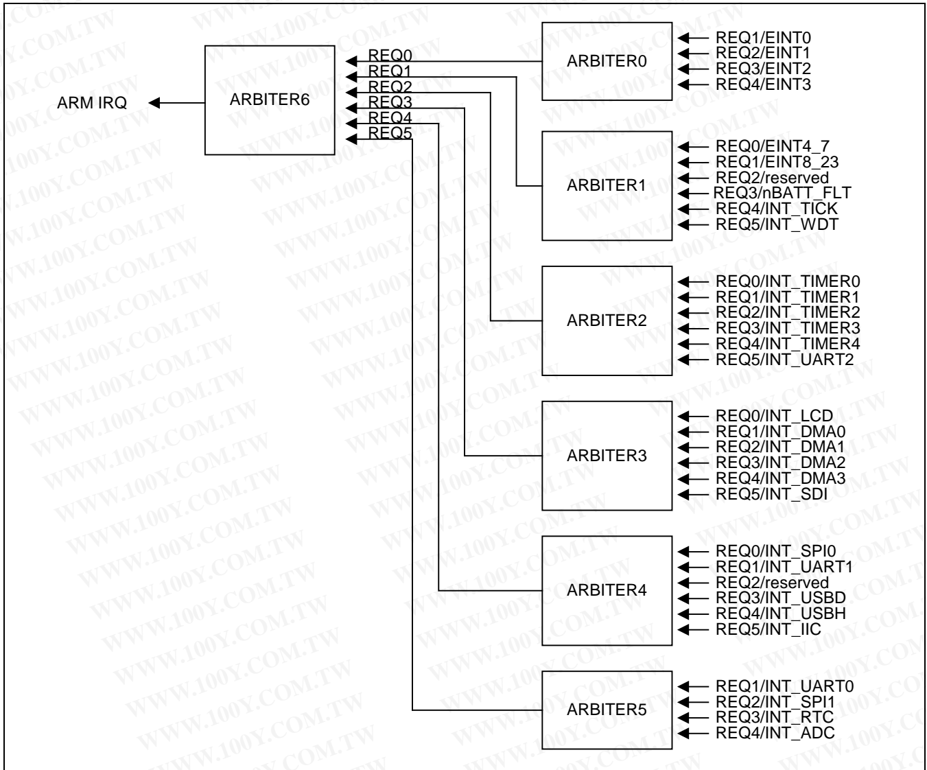
Figure 14-1. Priority Generating Block
