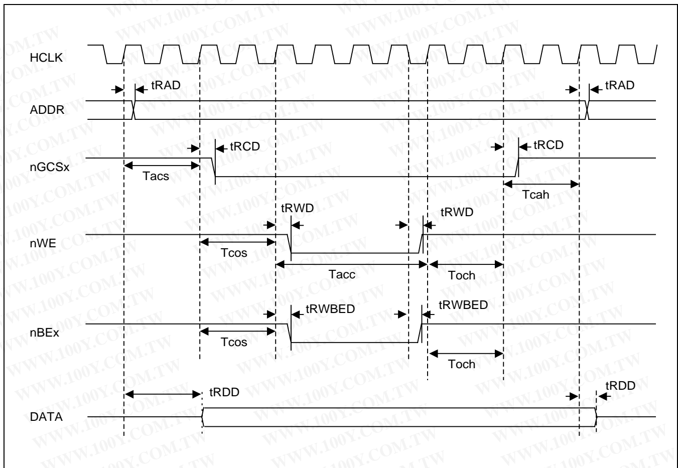
Figure 24-9. ROM/SRAM WRITE Timing (I) ( T_{acs}=2, T_{cos}=2, T_{acc}=4, T_{och}=2, T_{cah}=2, PMC=0, ST=0 )
