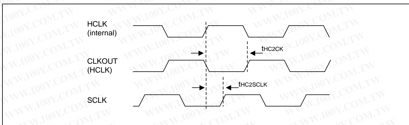
Figure 24-4. HCLK/CLKOUT/SCLK in case that EXTCLK is used
