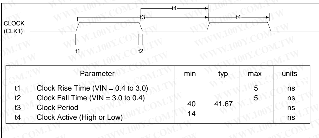
FIGURE 8 - CLOCK TIMING
