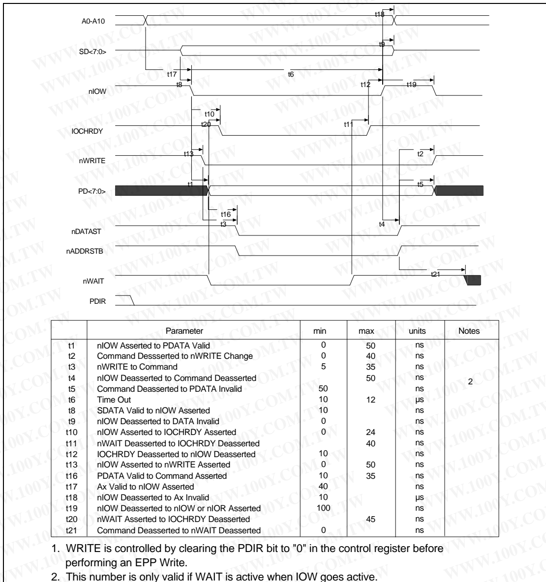
FIGURE 15 - EPP 1.7 DATA OR ADDRESS WRITE CYCLE
