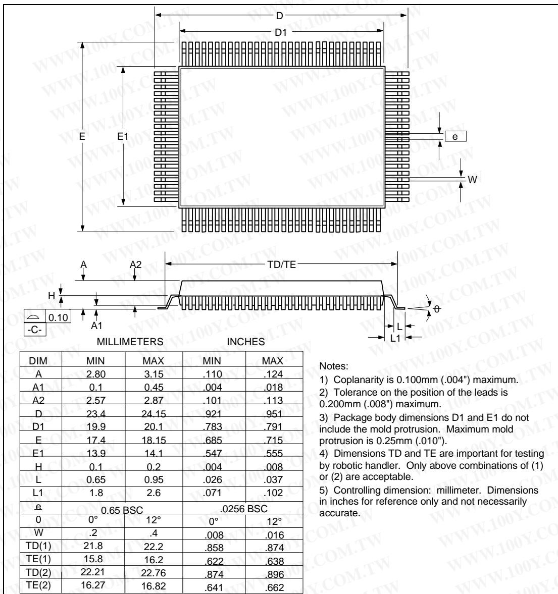
FIGURE 20 - 100 PIN QFP
