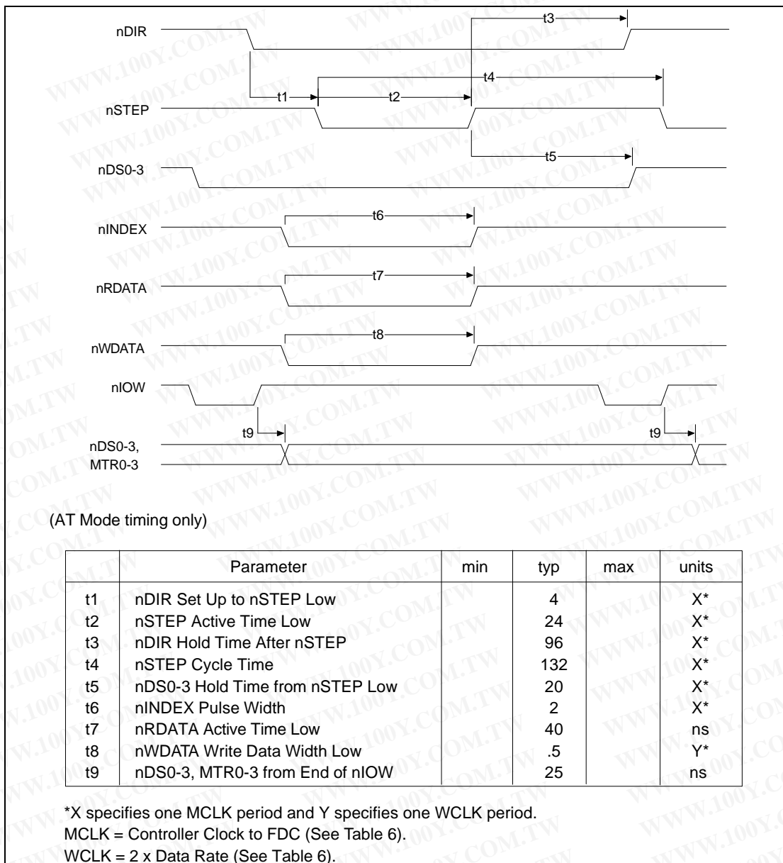
FIGURE 9 - DISK DRIVE TIMING
