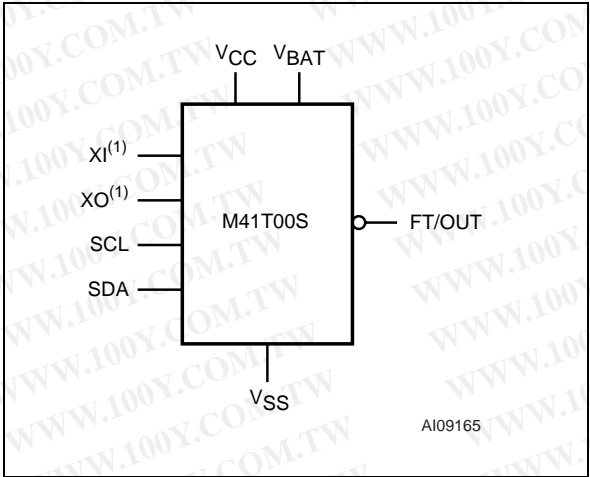
Figure 2. Logic Diagram
