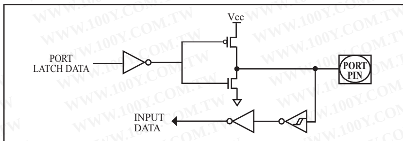
Push-pull output
