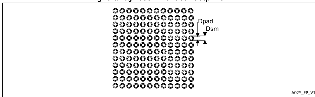
Figure 79. UFBGA144 - 144-pin, 10 x 10 mm, 0.80 mm pitch, ultra fine pitch ball grid array recommended footprint
